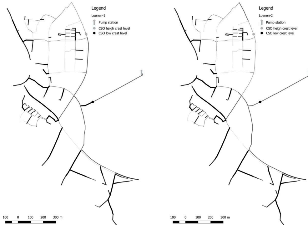
Figure 14. Degree of criticality for Loenen-1 ( left ) and Loenen-2 ( right ): the darker the line, the more critical the conduits. A part of the conduits has the same degree of criticality, but the conduits south of the high overflow structure have a different degree of criticality. In Loenen-2, these conduits are less important because in the case these conduits are blocked the water can flow to the high overflow structure which is not possible in the Loenen-1 system.
