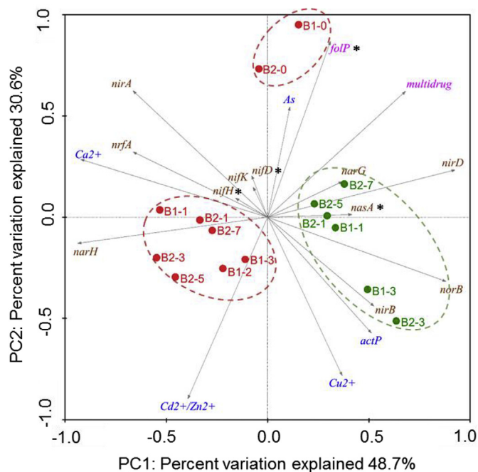
Fig. 9. PCA result of predicted functional genes related to nitrogen (brown), metal (blue) and sulfonamide (pink) metabolism and transport in RBF before (green dots) and after (red dots) sulfonamides stress. Relative abundance with significant difference were labeled with * ( p < 0.05 ). (For interpretation of the references to colour in this figure legend, the reader is referred to the Web version of this article.)
