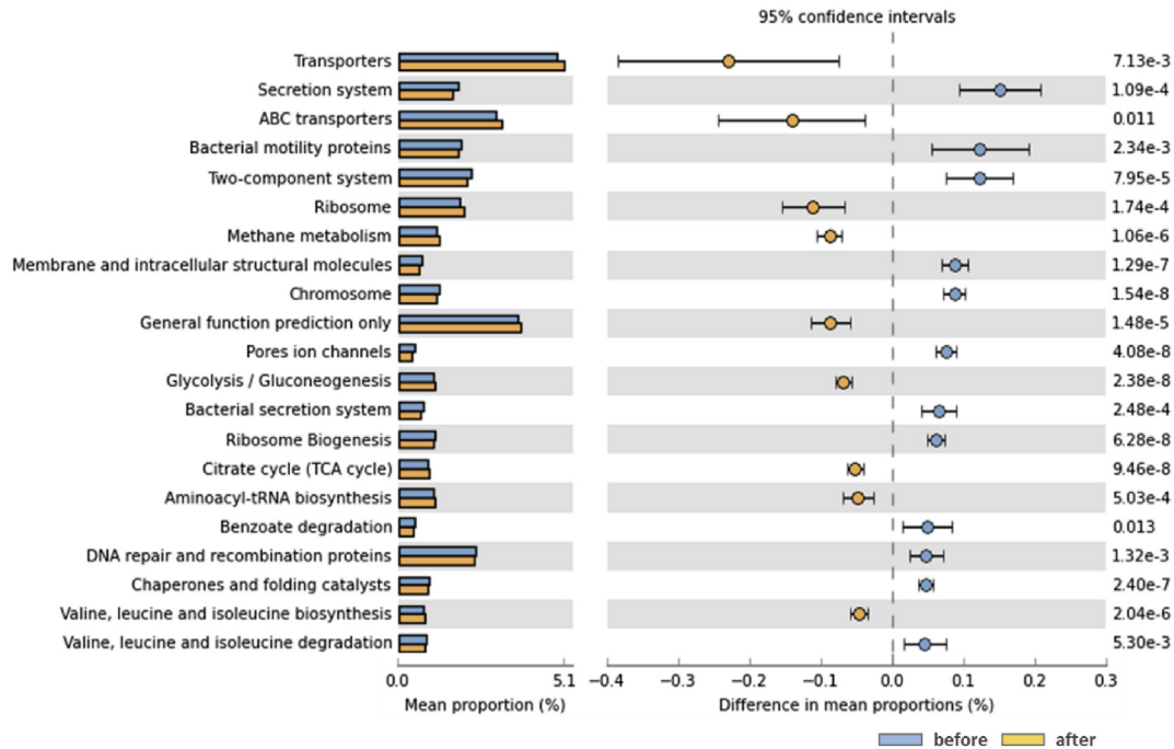
Fig. 8. Metabolism function proportion and diversity before and after SNs pressure ( p < 0.05 ).
