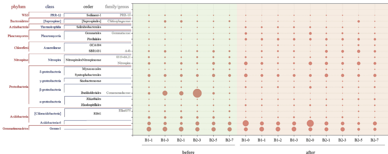
Fig. 4. Relative abundance of main bacteria taxa (>1% relative abundance, 100% occupancy) at the identified level before and after SNs stress (sample B1-1 represent RBF system B1 at the depth of 1 m).
