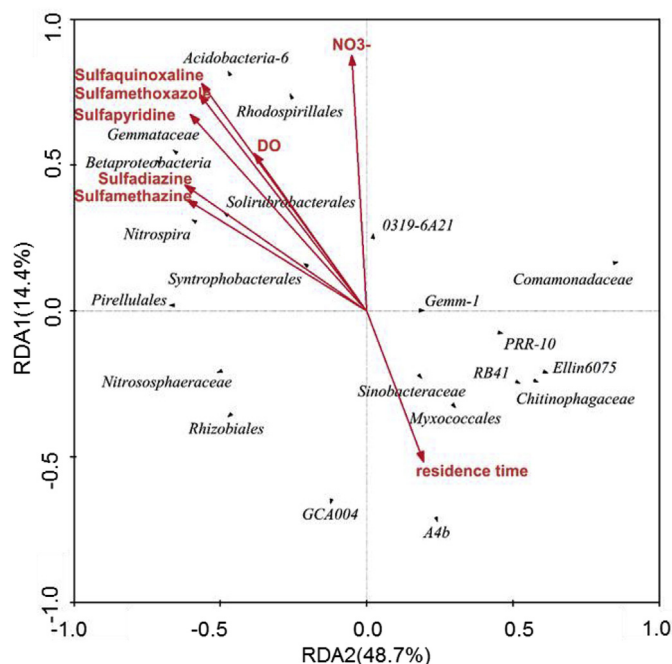
Fig. 7. Redundancy analysis of environmental factors with microbial species in RBF systems.
