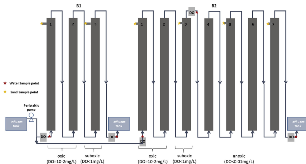
Fig. 1. RBF column set-ups.
