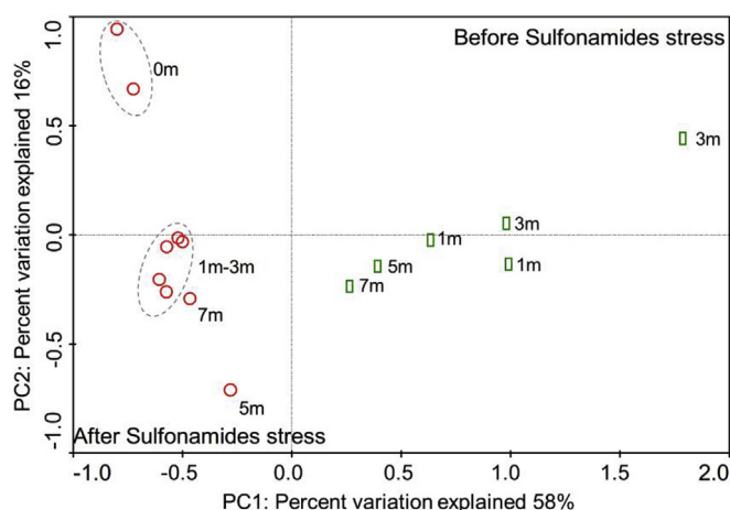
Fig. 5. PCA result of microbial taxonomy in B1 and B2 (Green rectangular and red dot represent sample collected before and after SNs addition respectively. X m represent the flow depth). (For interpretation of the references to colour in this figure legend, the reader is referred to the Web version of this article.)
