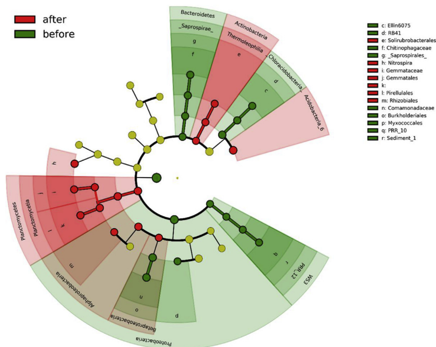
Fig. 6. LEfSe analysis results (The green and red circle represent the enriched taxa in community before and after sulfonamides pressure, yellow circles represent taxa with no significant differences between two communities). The phylum, class, order, family, and genus levels are listed from inside to outside. (For interpretation of the references to colour in this figure legend, the reader is referred to the Web version of this article.)
