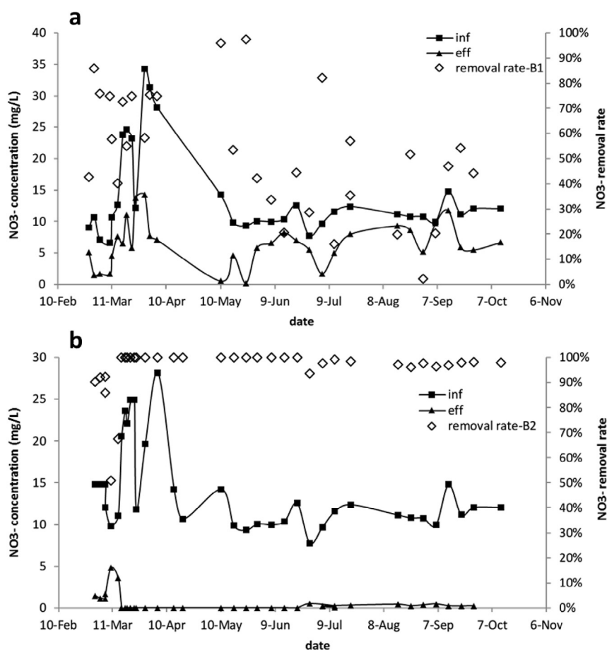
Fig. 2. Nitrate removal ratio in RBF systems B1 (a) and B2 (b).
