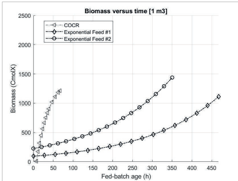
Figure 13. Predictions of biomass accumulation versus time using exponential feed strategy for 1 m 3 , comparing fed - batch strategies.
