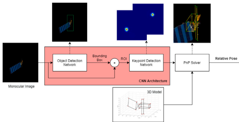
Fig. 12. Proposed CNN architecture and interface with the PnP solver.
