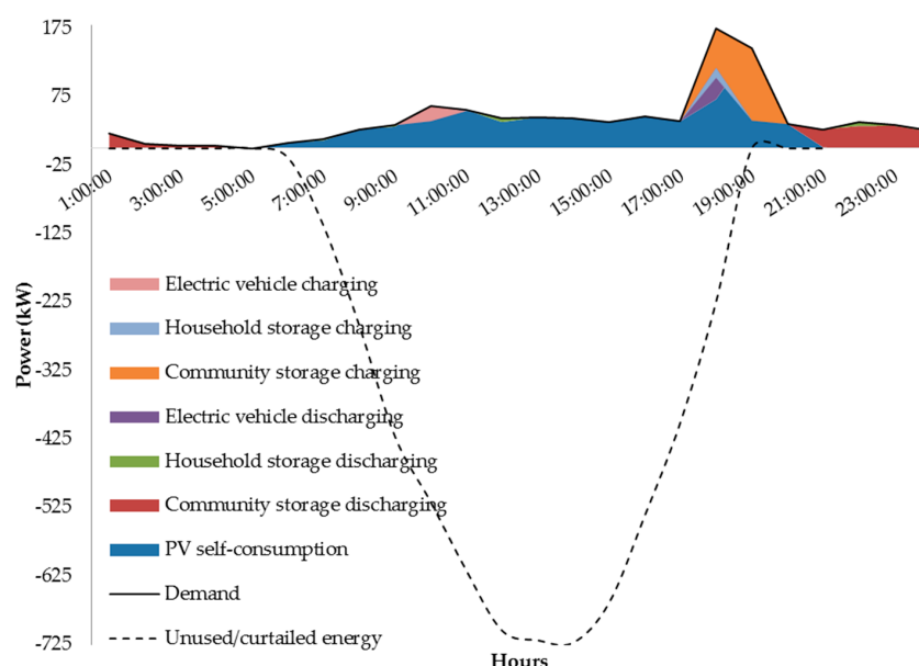
Figure 13. Energy balance on peak-day of May for the grid-defected ICES.
