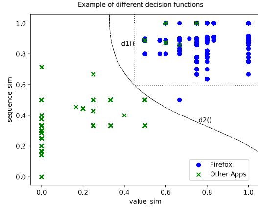
Figure 1: Distribution of messages after they have been compared with the fingerprint of Firefox. Crosses represent messages from applications other than Firefox. Dots represent messages from Firefox. The straight and dashed lines represent two possible decision functions.
