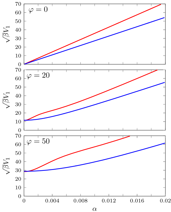
Fig. 9 Stability bounds for the full system of three modes \{5, 3, 2\} — and the truncated system of two modes \{3, 2\} —. Stability region in (\alpha, \sqrt{B}V_1) plane is below each curve
