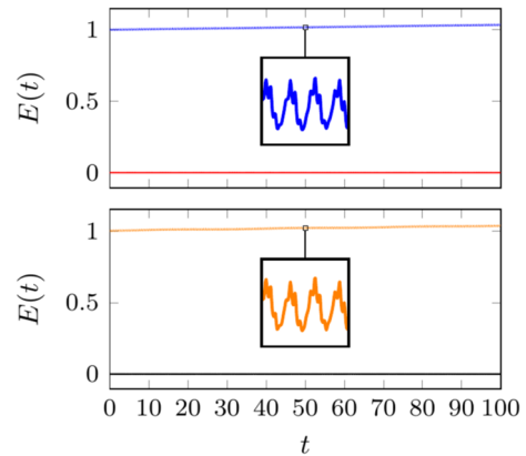
Fig. 17 Time evolution of E_1(t) (blue), E_3(t) (red), total energy E_{\text{total}}(t) (orange), and the energy of the remaining modes E_{\text{total}}(t) - E_1(t) (black)
