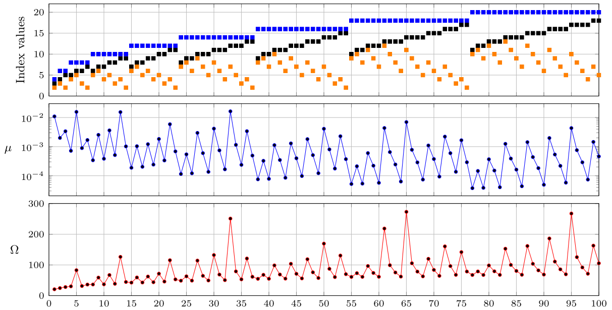
Fig. 6 Contributing modes to the first 100 coincidences: \omega_K + \omega_N = \omega_M , with corresponding \mu and \Omega values
