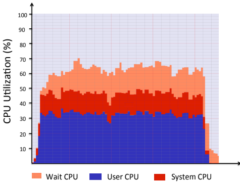
Figure 4.9: CPU Utilization of the cluster when Pi+Sort are in parallel executed by DARA
