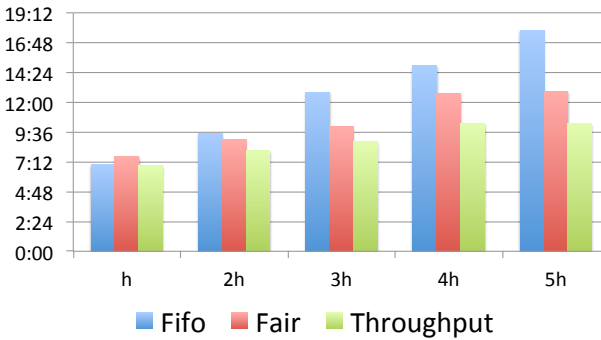
Figure 3.7: Overall application completion time in minutes (Y axis) on heterogeneous machines at PARC for different relative values of h = \frac{\theta_d}{\theta_c} . Disk load \theta_d is increased by increasing the replication number.
