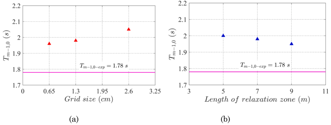
Fig. 10. Sensitivity of the numerically modelled spectral wave period T_{m-1,0} (a) with the grid size: 0.65 cm \times 0.65 cm, 1.3 cm \times 1.3 cm, 2.6 cm \times 2.6 cm (from left to right) and (b) with the length of the inlet relaxation zone: 5 m, 7 m, 9 m (from left to right). The experimentally measured T_{m-1,0-exp} is 1.78 s.
