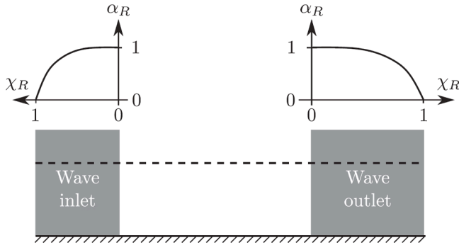
Fig. 4. Variation of \alpha_R(\chi_R) in relaxation zones (from Jacobsen et al., 2012).
