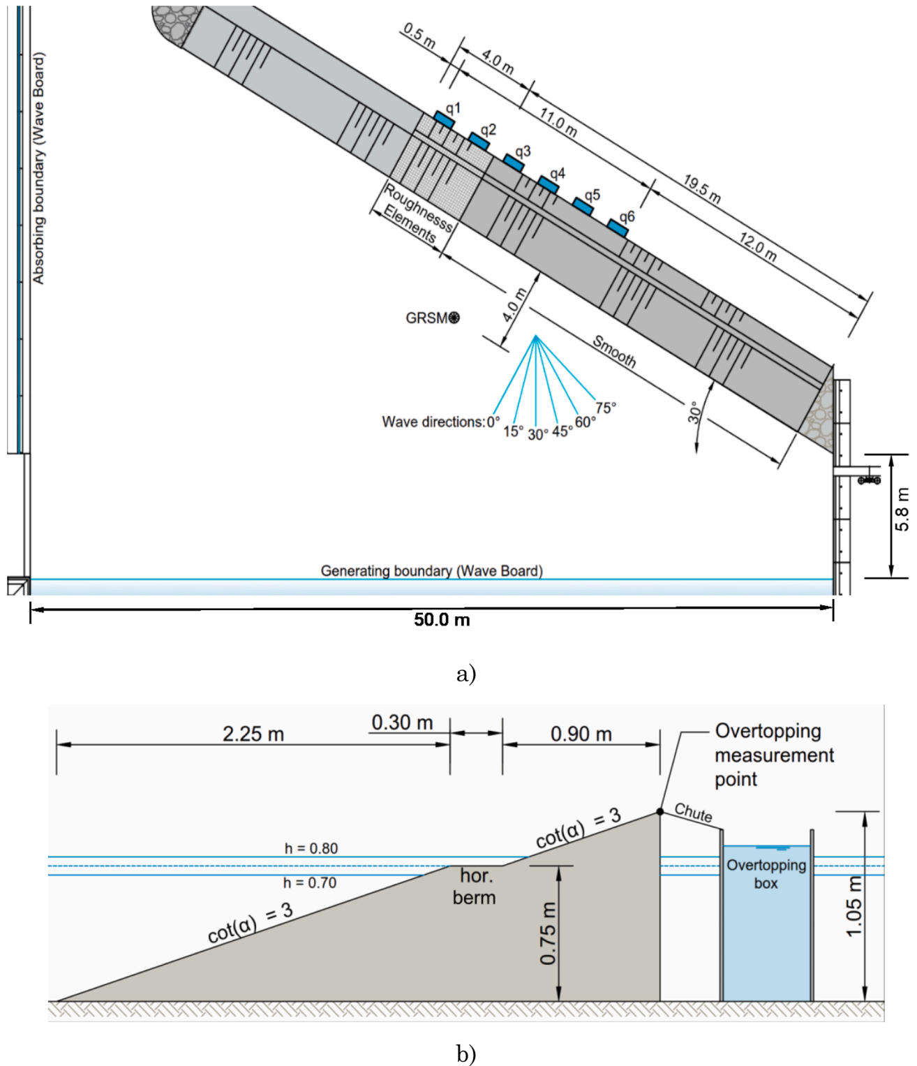
Fig. 6. Three-dimensional physical model set-up with a) layout of the model in the wave basin and b) tested cross-section (from Van Gent, 2020).
