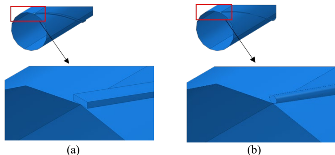
Fig. 7 Model with rectangular (a) and round (b) wire cross section
