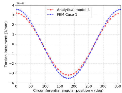
Fig. 13 Torsion increment for the round wire under analytical model and FE model
