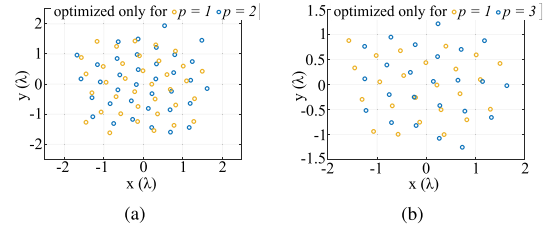
Fig. 6. Layout comparisons for single subset optimization. (a) 36 elements. (b) 24 elements.
