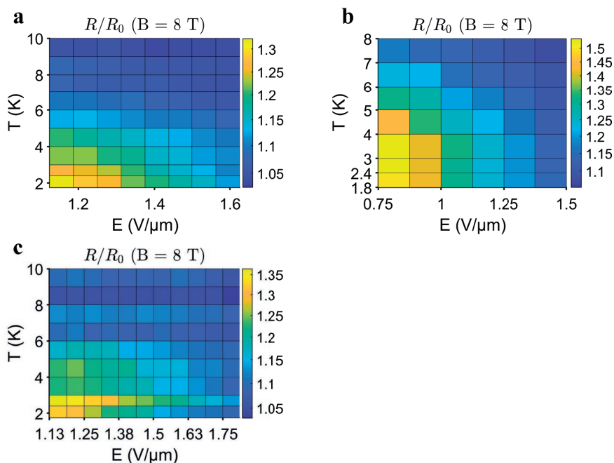
Figure S4: Colour maps of the magneto-resistive effect for the three segments. a-c correspond to the segments 1, 2 and 3, respectively. The data plotted in Fig. S1 can be used to construct a colour map, with on the vertical axis the temperature, T . Each rectangle is coloured by the average of the four data points at its corners. On the horizontal axis, the electric field, E (voltage divided by segment length, see Table S2). The colour indicates the strength of the relative magneto-resistance, R/R_0 at high magnetic field ( B = 8 T).
