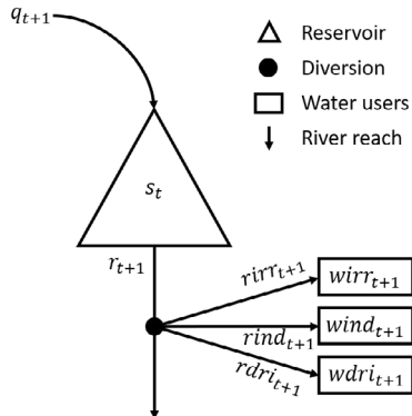
Fig. 3. An illustrative example of a single-reservoir subsystem.
