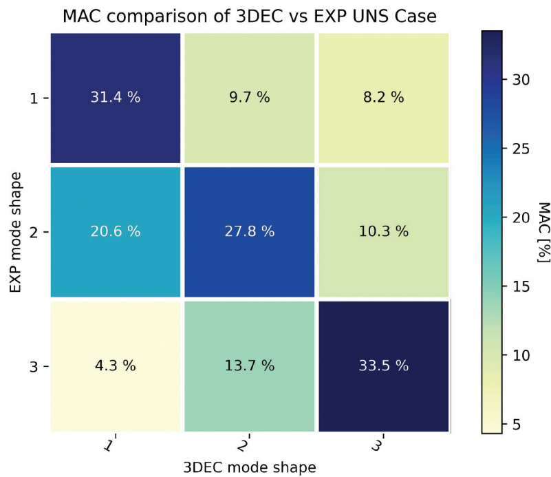
Figure 22. MAC Comparison of 3DEC and EXP for the UNS-POST case.
