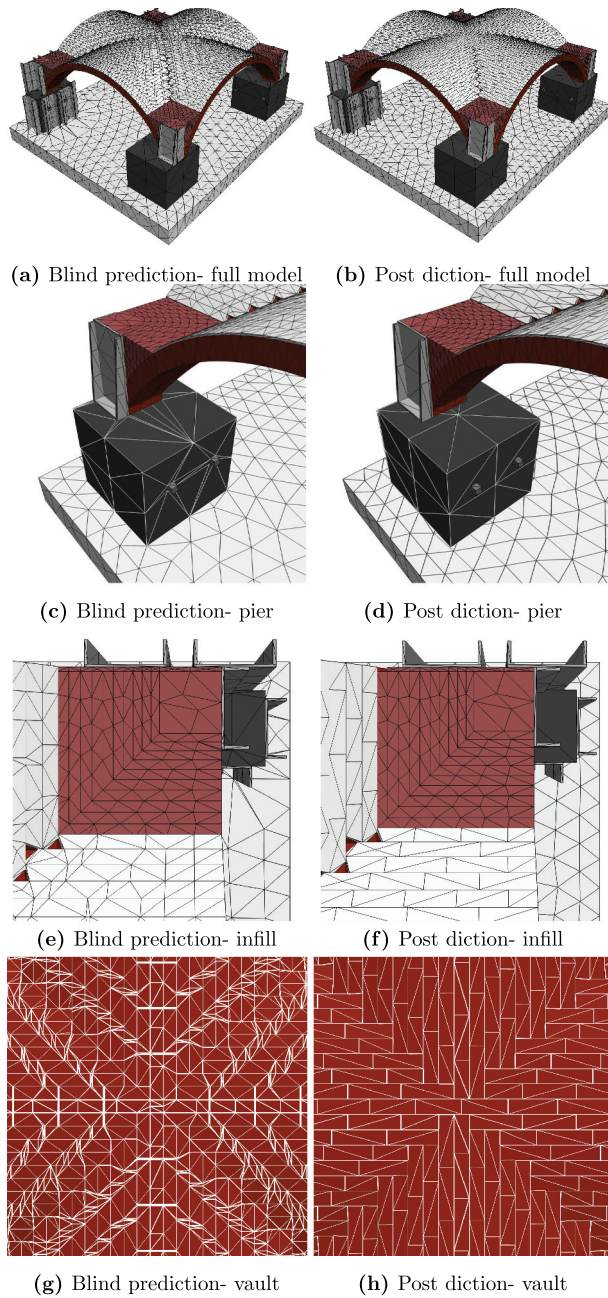
Figure 19. Mesh refinement.
