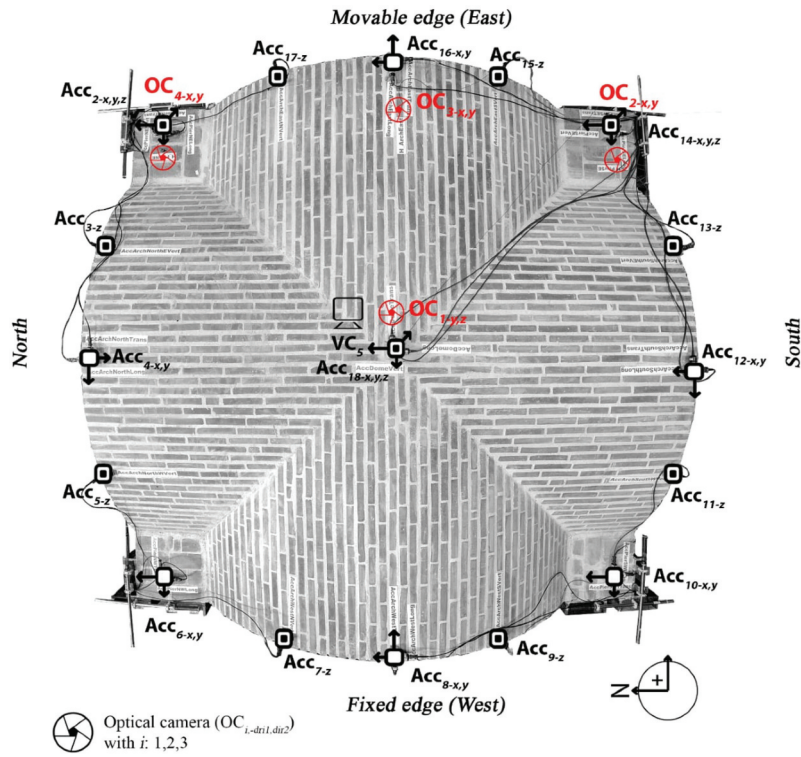
Figure 2. Instrumentation setup for the SERA cross-vault experiment (Bianchini et al. 2023).
