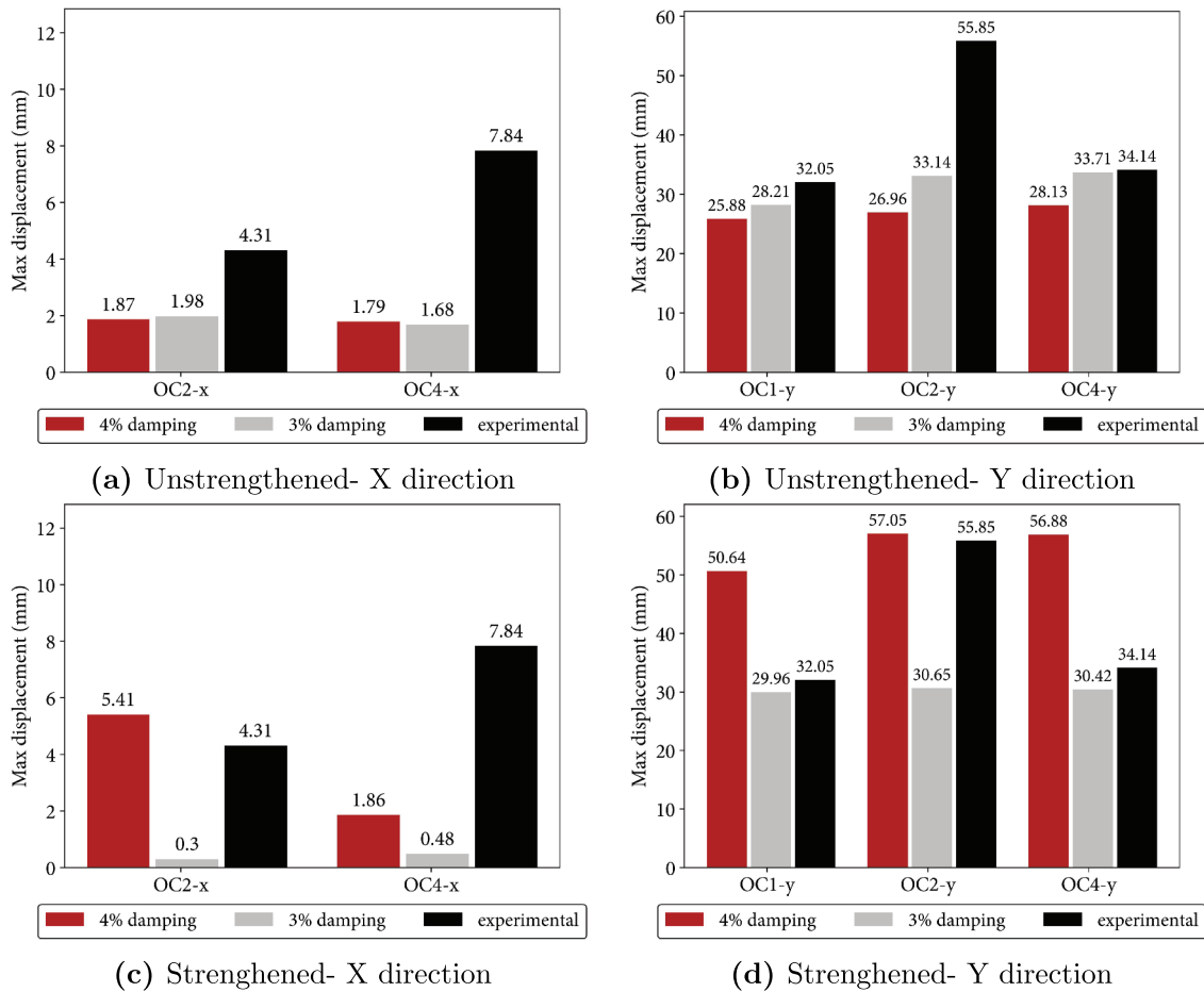
Figure 20. Damping calibration.
