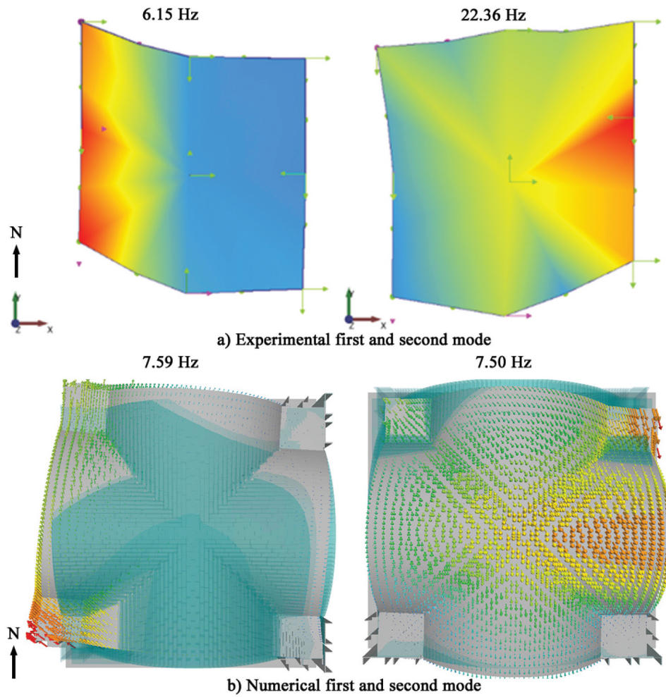
Figure 29. Comparison of eigenvalue analysis and mode shapes for the reinforced numerical model and experiment (strengthened case).
