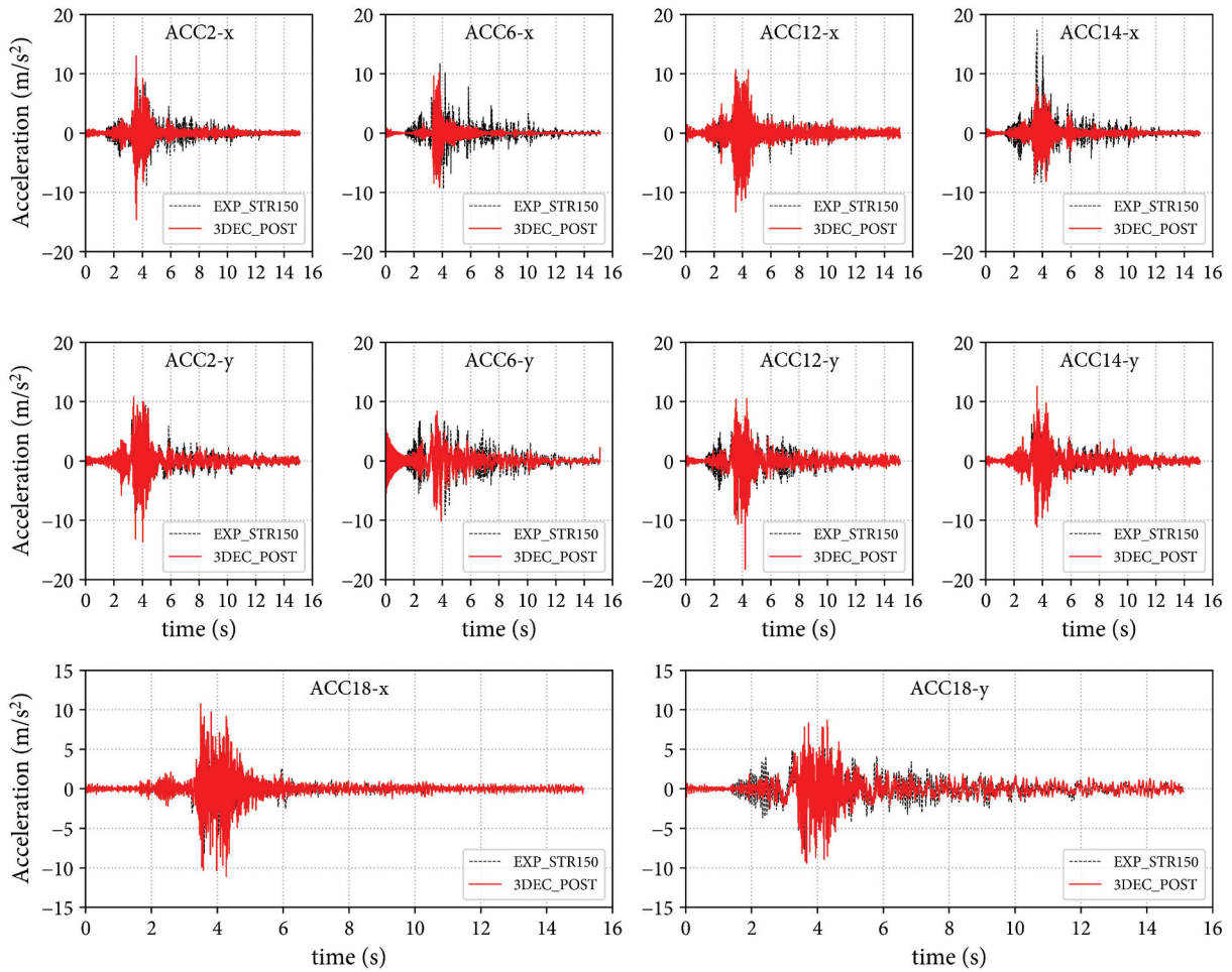
Figure 34. Comparison of post-diction acceleration responses at selected accelerometers on the 150% load increment (strengthened case).
