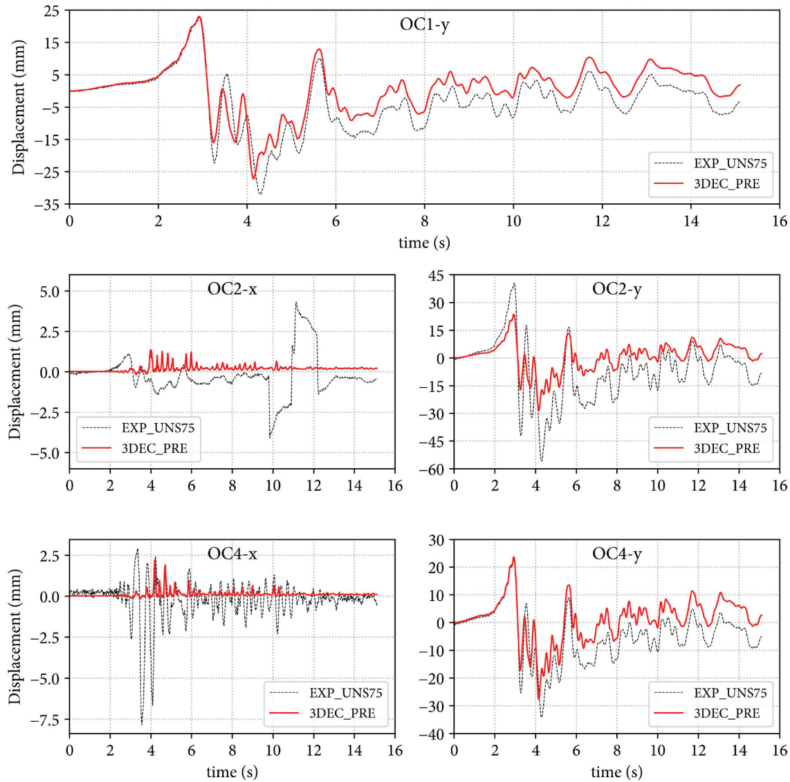
Figure 14. Experimental and numerical comparison of displacement responses at each optical camera at 75% load increment (unstrengthened case).
