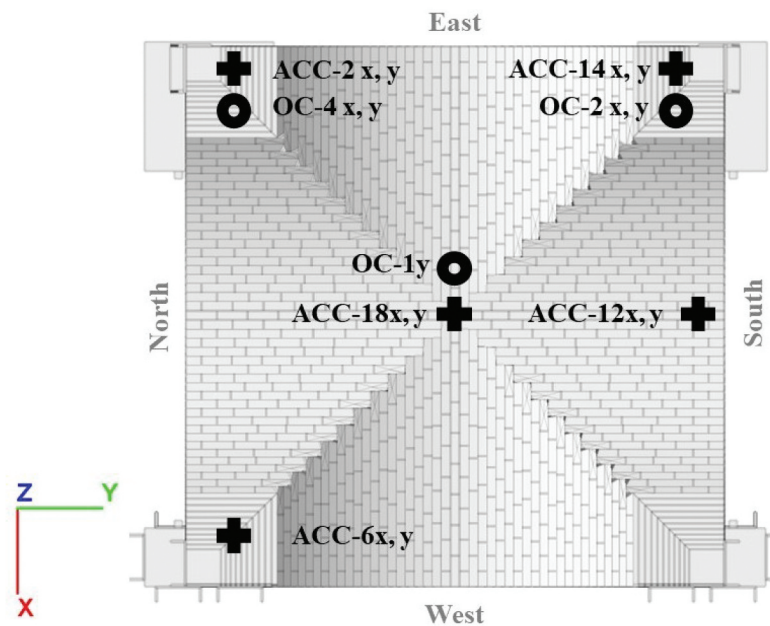
Figure 9. Accelerometer (ACC) and optical camera (OC) placement.
