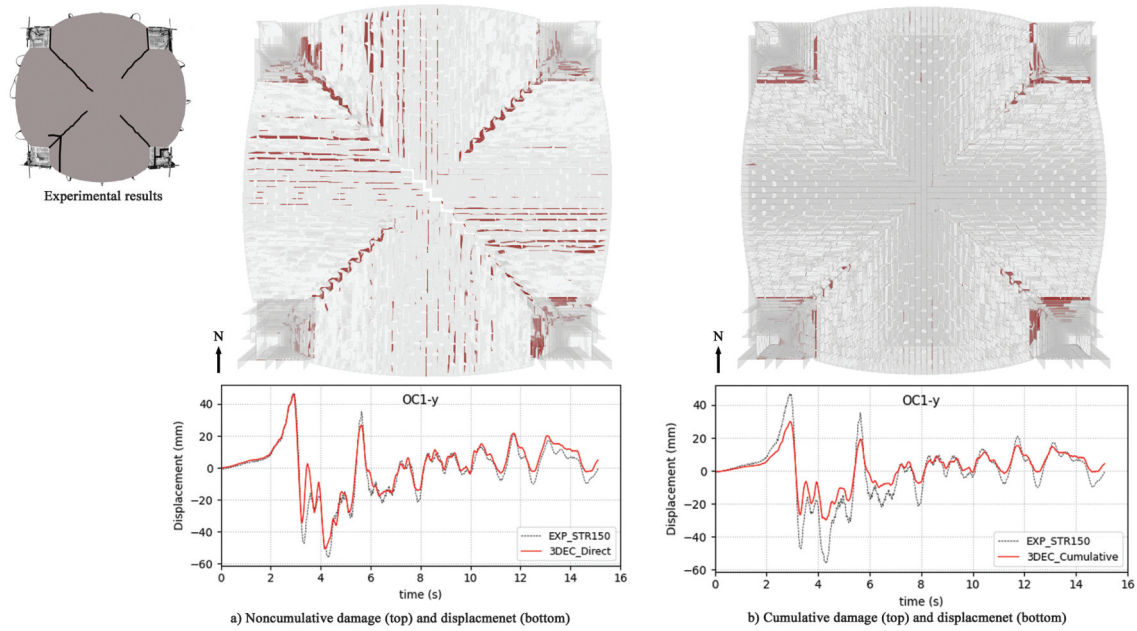
Figure 31. Comparison of cumulative and non-cumulative damage of the strengthened cross vault at the 150% load increment, with the reinforcement hidden.
