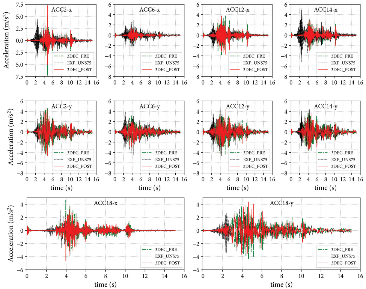
Figure 28. Comparison of post-diction acceleration responses at selected accelerometers on the 75% load increment (unstrengthened case).
