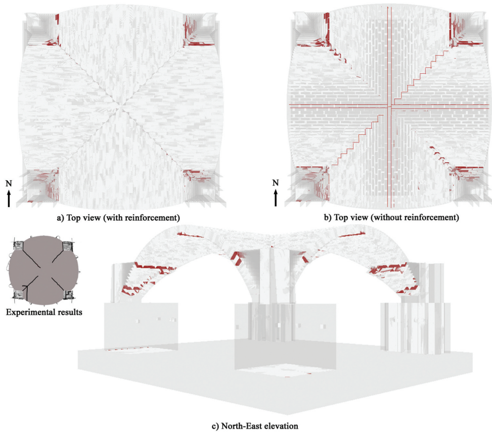
Figure 32. Cumulative damage in the strengthened model at the 150% load increment.
