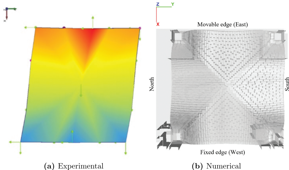
Figure 12. First mode shape comparison between experimental and numerical analysis at prediction stage.
