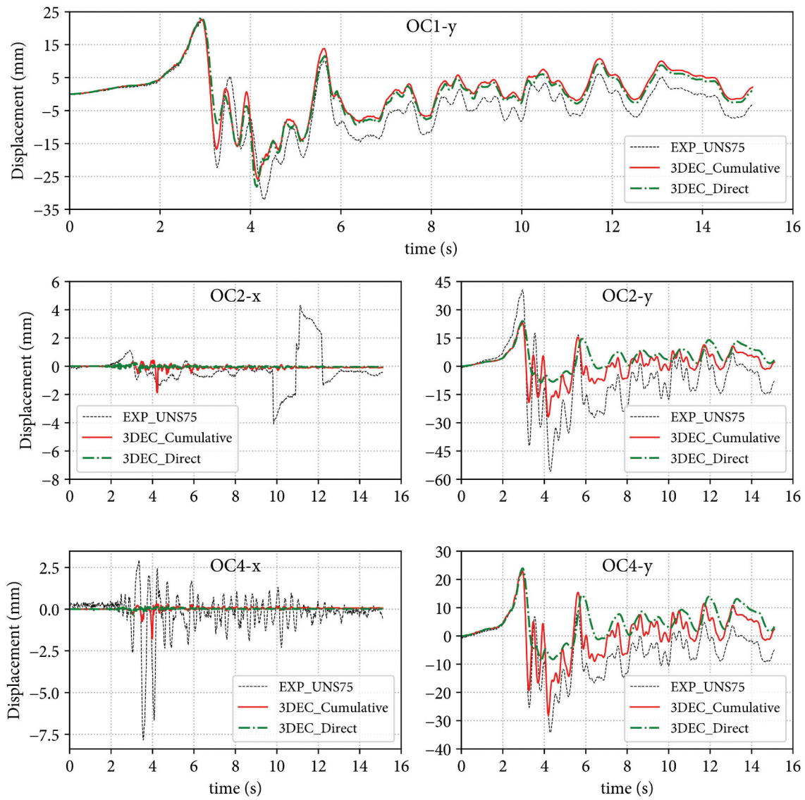
Figure 24. Comparison of displacement responses between direct and incremental.
