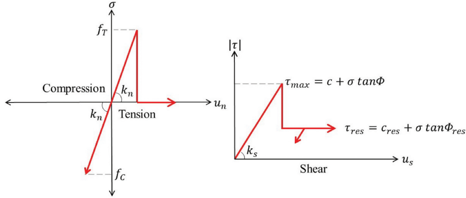
(b) Mohr-Coulomb joint model
