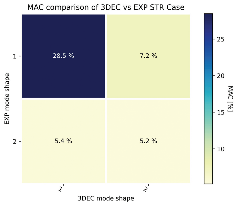
Figure 30. MAC Comparison of 3DEC and EXP for the UNS case.
