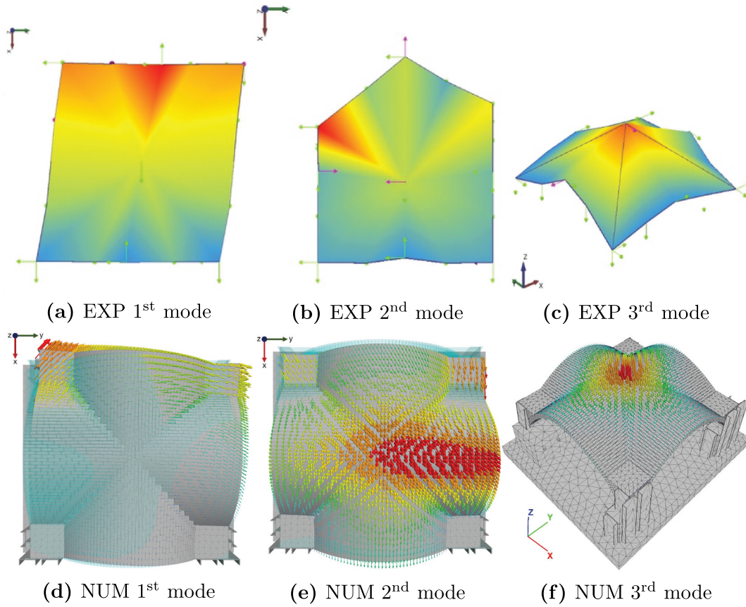
Figure 21. Comparison of mode shapes.
