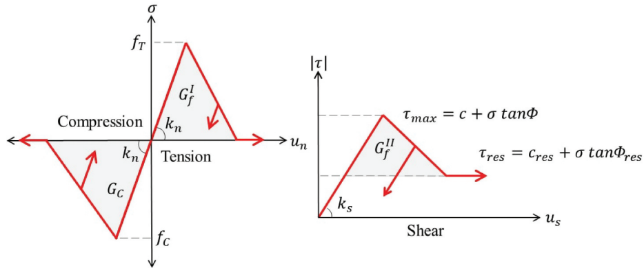
(c) Fracture energy-based elasto-softening joint model
