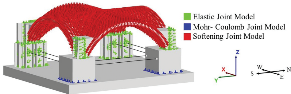
Figure 10. Definition of joint constitutive relations.
