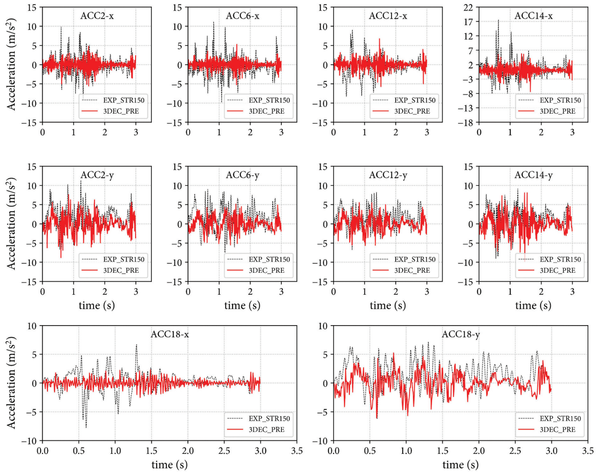
Figure 18. Comparison of acceleration responses at selected accelerometers at 150% load increment (strengthened case).
