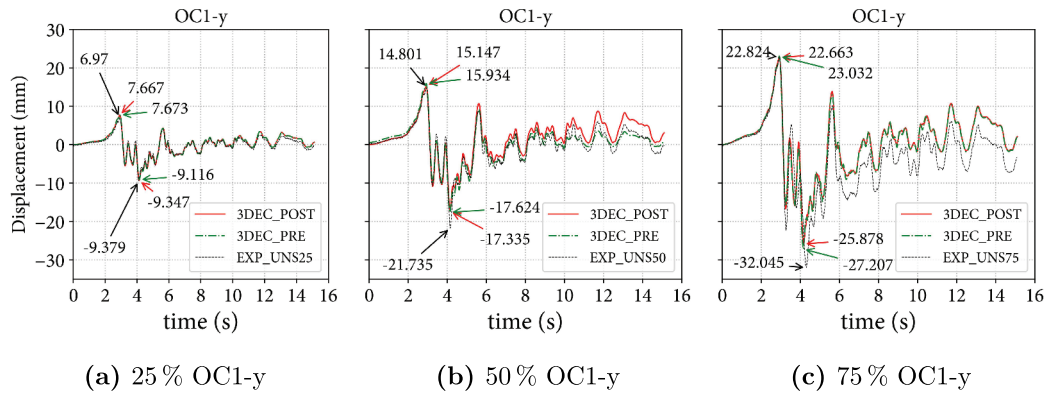
Figure 26. Comparison of displacement evolution at OC1-y.
