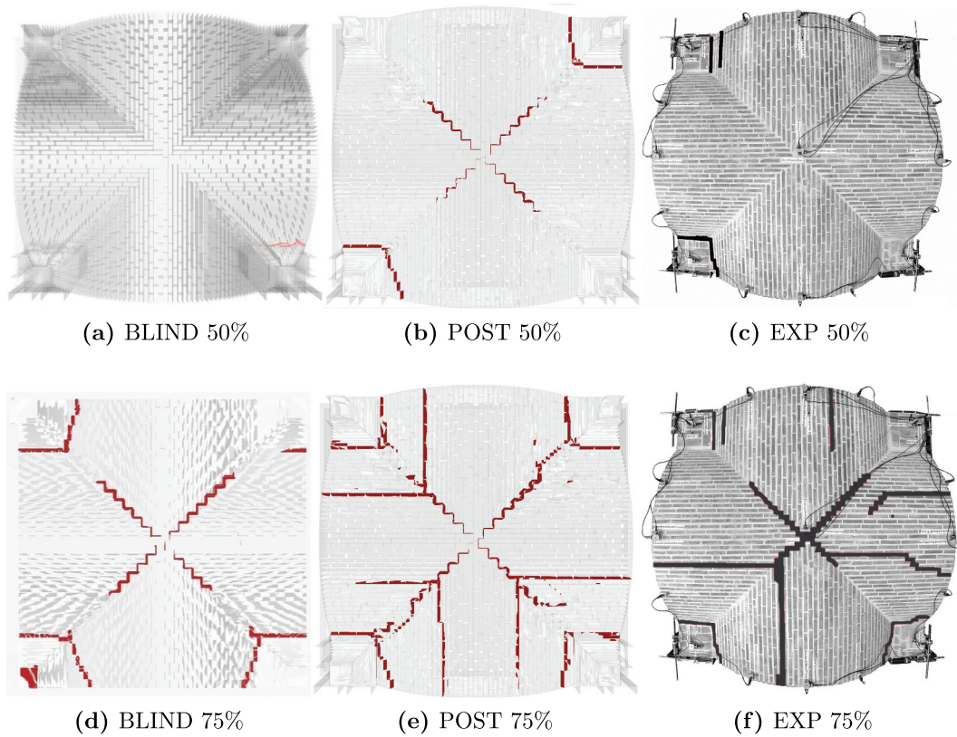
Figure 23. Comparison of crack patterns of the unstrengthened vault between blind prediction, post-diction, and experiment at selected load increments.
