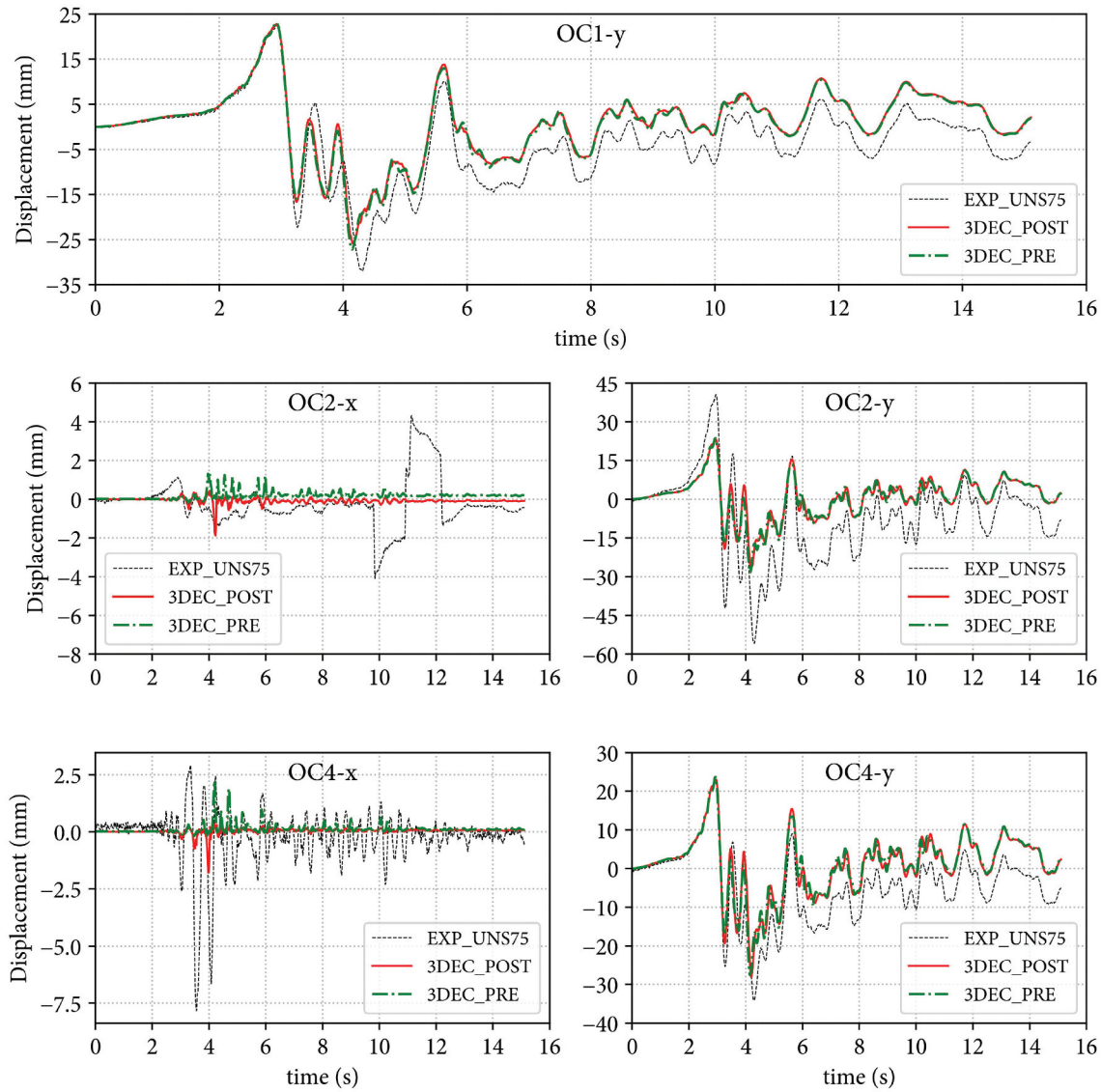
Figure 27. Comparison of displacement responses at each optical cameras on the 75% load increment (unstrengthened case).
