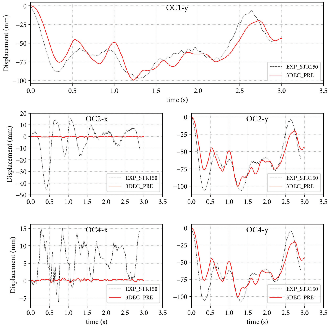
Figure 17. Comparison of displacement responses at each optical camera at 150% load increment (strengthened case).
