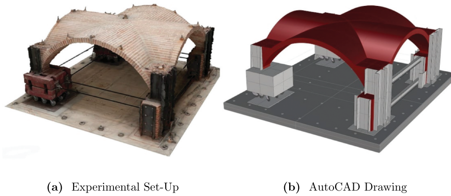
Figure 3. Modeled cross-vault (Bianchini et al. 2023).
