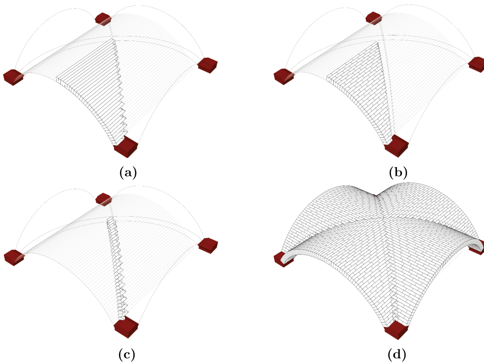
Figure 4. Parametric geometry generation a) course discretization b) fine discretization c) groin generation d) assembly of full vault.
