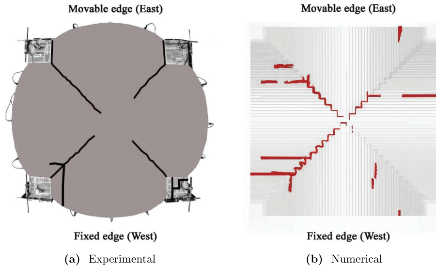
Figure 16. Comparison of strengthened crack patterns at the vault extrados.
