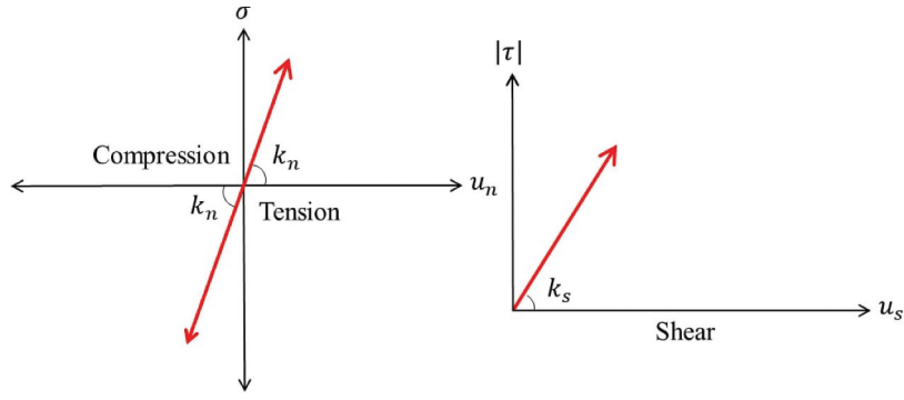
(a) Elastic joint model
