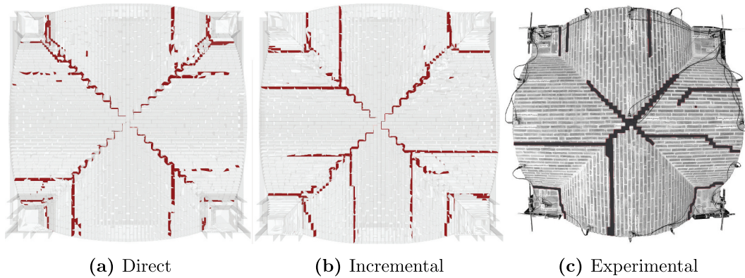
Figure 25. Comparison of crack pattern between direct and incremental seismic load.
