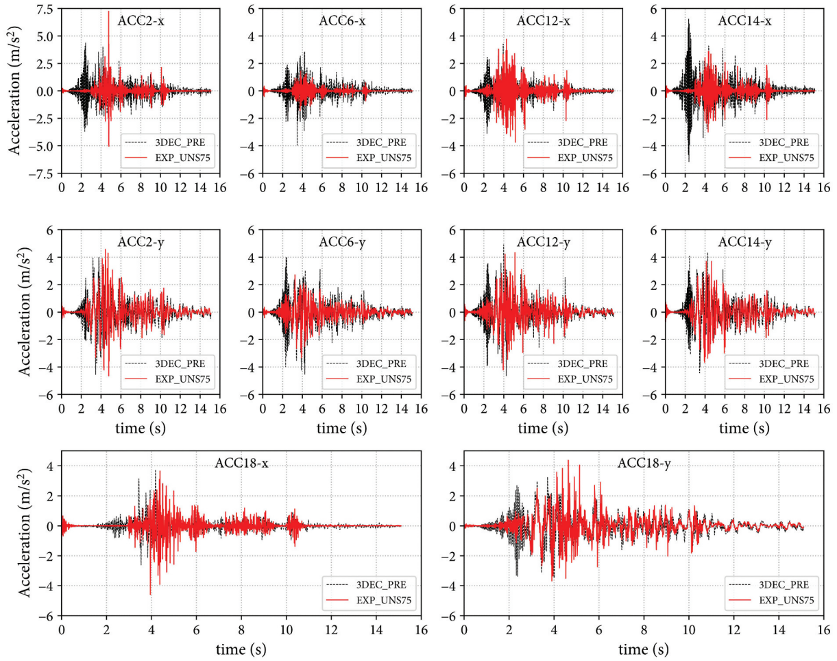
Figure 15. Comparison of acceleration responses at selected accelerometers at 75% load increment (unstrengthened case).
