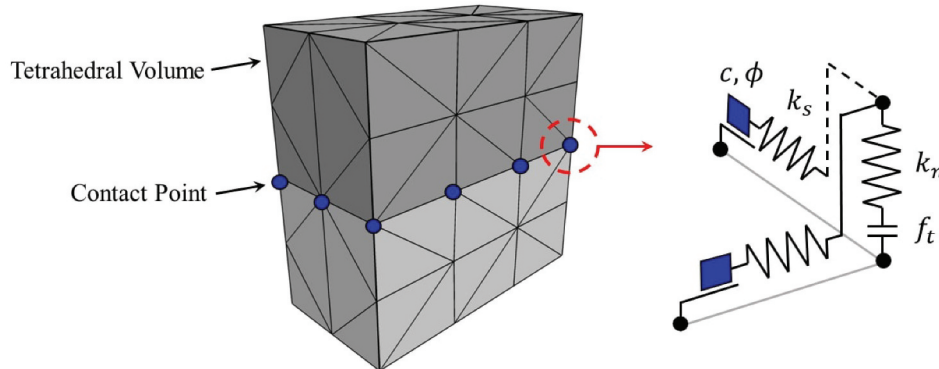
Figure 5. Representation of contact between blocks in DEM.
