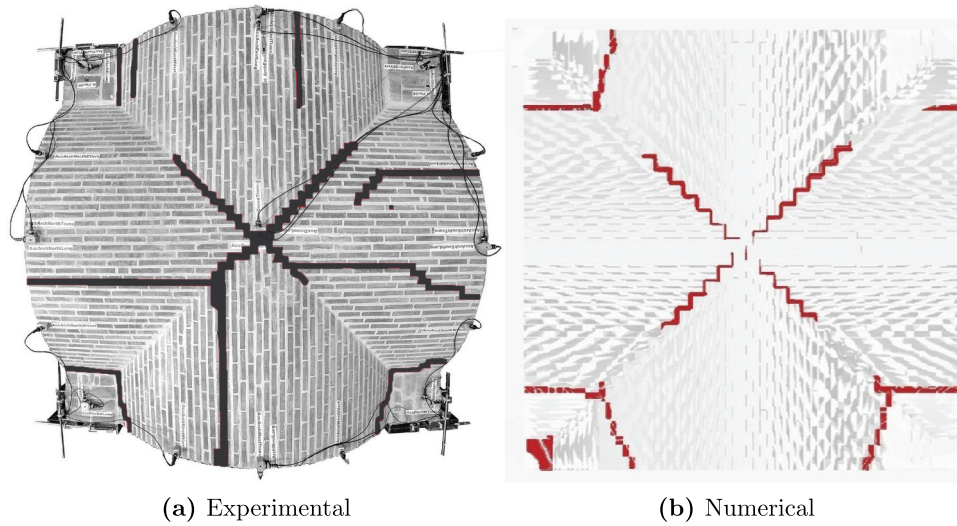
Figure 13. Comparison of (a) experimental (Bianchini et al. 2023) and (b) numerical crack patterns at the vault extrados.
