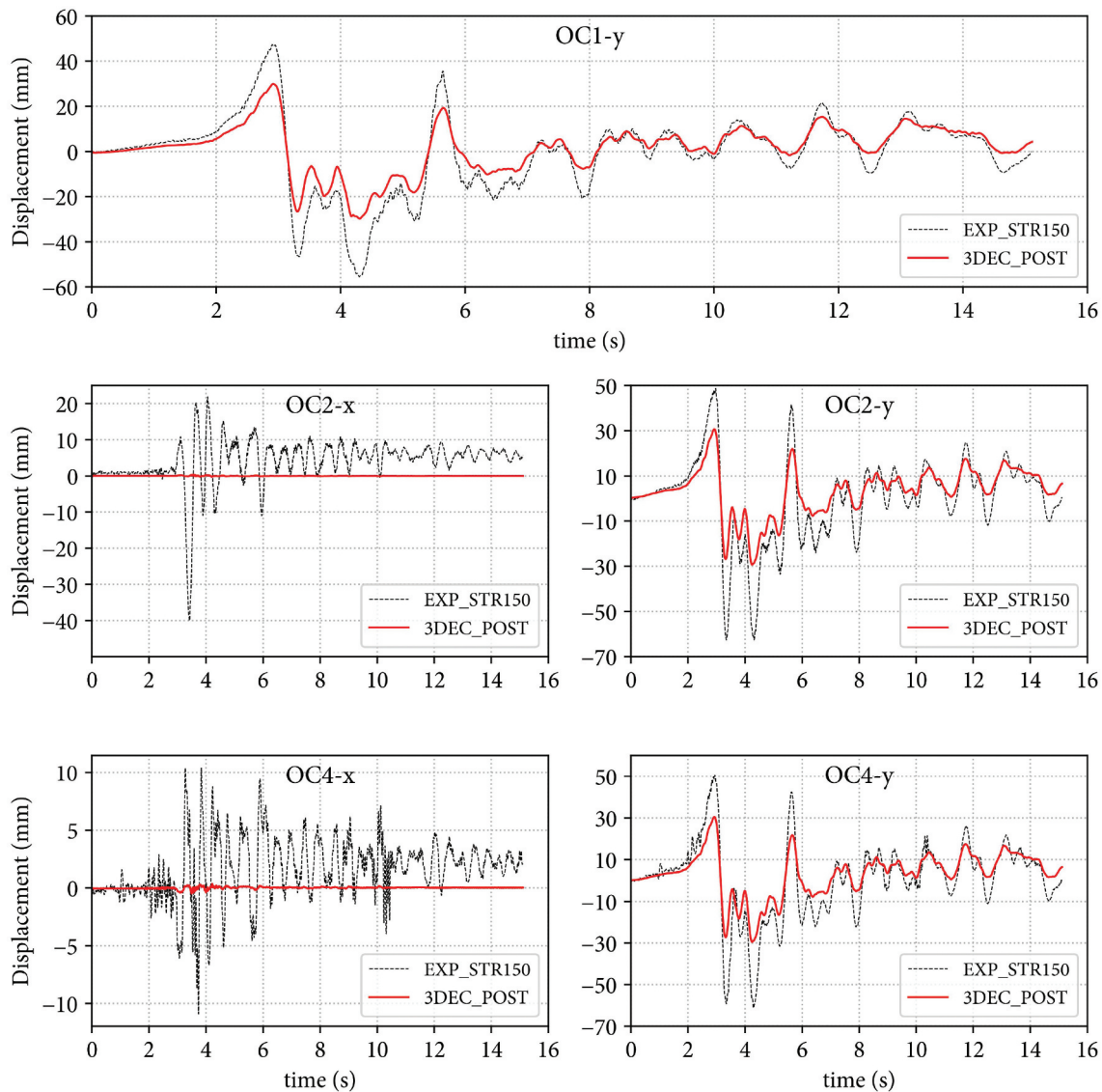
Figure 33. Comparison of displacement responses at each optical cameras on the 150% load increment (strengthened case).
