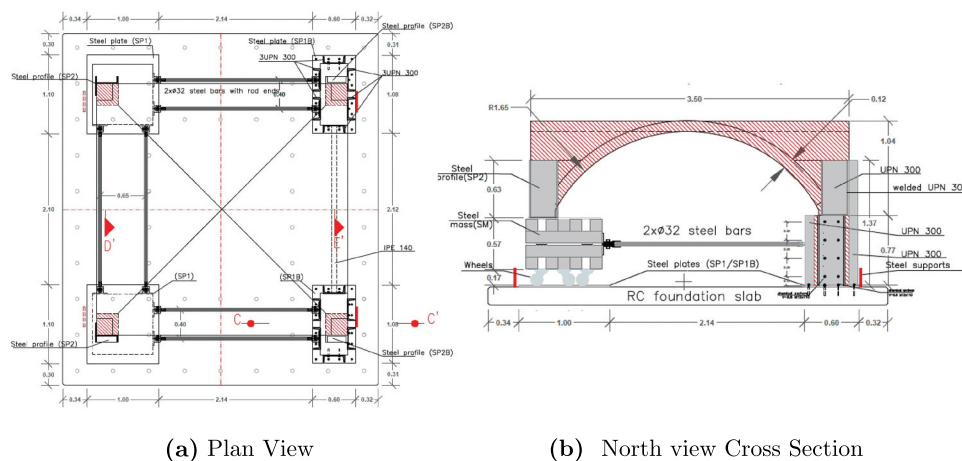
Figure 1. Experimental specimen detailed specifications (Bianchini et al. 2023).
