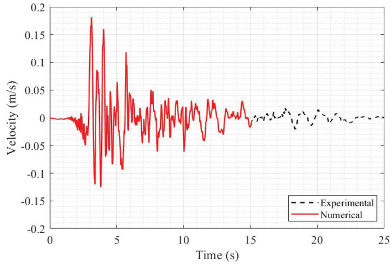
Figure 8. Experimental and truncated numerical velocity time history (L'aquila 75%).
