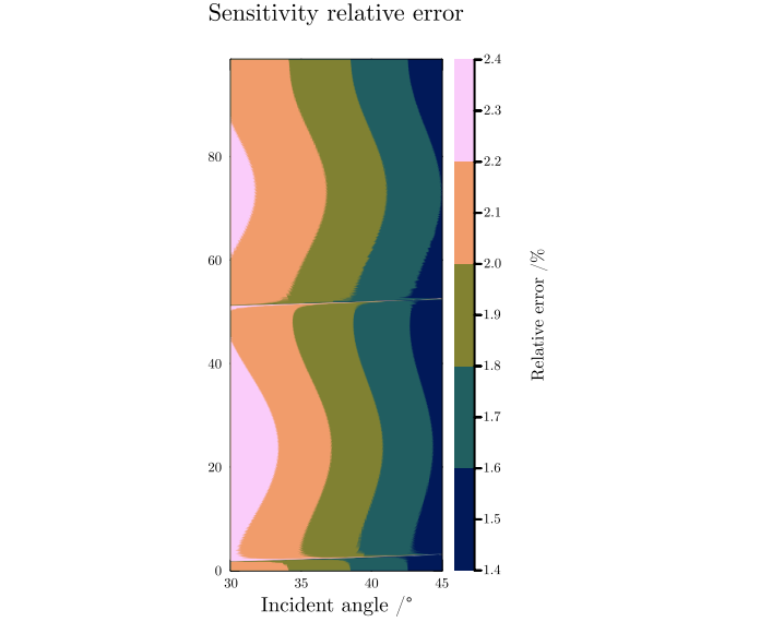
Fig. 11. The relative error of the sensitivity calculated using the wavenumber method with respect to the conventional sensitivity expression. For the expression of the sensitivity the incidence angle is computed according to (47) and the scaling of the wavelength described in (46) is omitted. A scaling factor of 2, corresponding to a monostatic system, is used instead.
