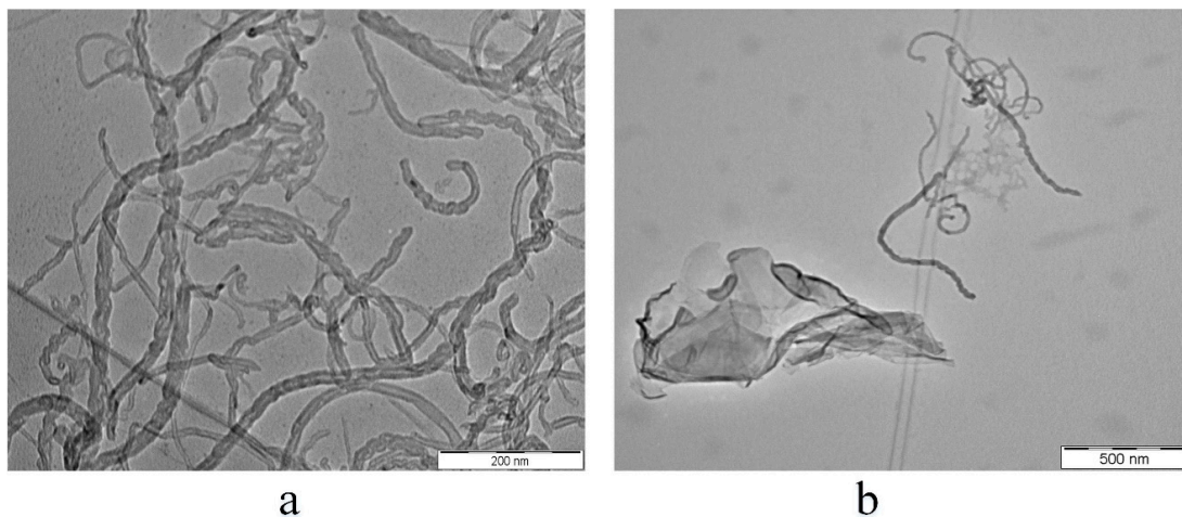
Figure 2. TEM images of (a) MWCNTs/water nanofluid and (b) MWCNTs/GNPs hybrid nanofluid.
