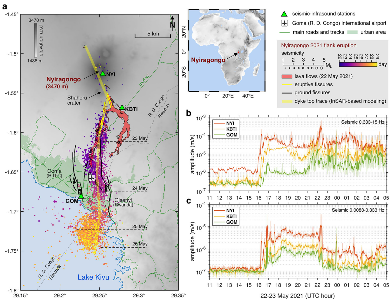
Fig. 1 | The May 2021 Nyiragongo flank eruption. a Map of Africa situating Mount Nyiragongo and zoom into the study area. Local stations (KivuSNet network 30 ) with co-located seismic and infrasound sensors are depicted as green triangles. Data for the Nyiragongo 2021 flank eruption 35 are the seismic events over time (blue to yellow from 22 to 28 May 2021, with marker size corresponding to the magnitude between 1 and 5, minimum latitudes along the path of the dyke at 00:00 UTC on 23, 24, 25 and 26 May are indicated by horizontal black dashed lines); the lava flows (red area); the eruptive fissures (yellow lines); the ground fissures detected from Interferometric Synthetic Aperture Radar (InSAR) (black lines); the dyke top trace connected to eruptive fractures (thick
