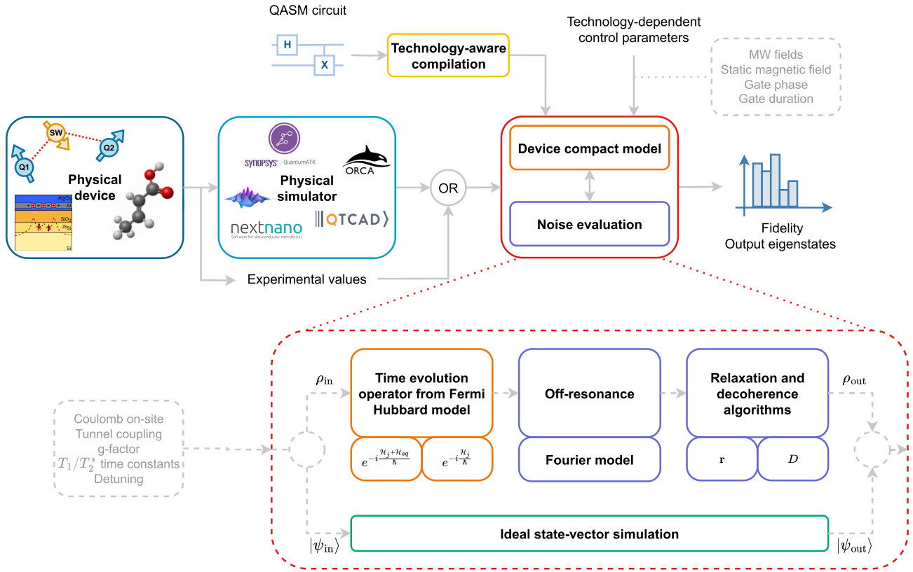
FIGURE 8. Integration of the quantum dot compact model in the quantum simulation toolchain. The symbol \mathcal{H}_{sq} refers to Equation (17); \mathcal{H}_j to one between Equation (17) and Equation (19); r is the relaxation vector of Equation (36) and D is the decoherence matrix of Equation (34).
