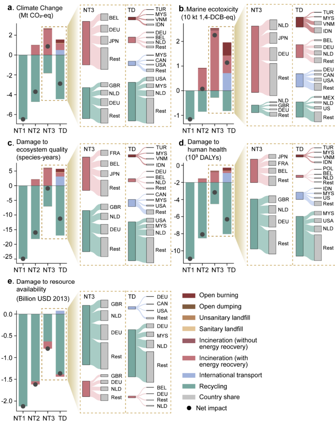
Figure 2. Environmental impacts of plastic waste trade in 2022 under four scenarios by waste treatments (breakdown by the top 3 countries and the rest between NT3 and TD scenarios). The environmental impacts are covered by two midpoint and three end point impact categories: climate change (a), marine ecotoxicity (b), damage to ecosystem quality (c), damage to human health (d), and damage to resource availability (e). Full country names matching their ISO country codes are given in Table S2.
