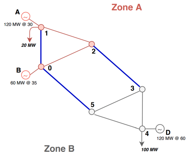
Fig. 2. Overview of a 2-zone test network with 3 critical branches (in blue). The nodes and branches belonging to Zone A are marked in red, those belonging to Zone B are marked in grey. Next to the generators in the figure, the reader can find their maximum available capacities in MW and day-ahead market bids in €/MWh.
