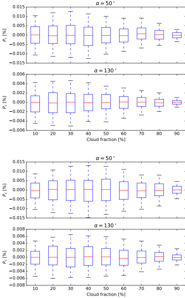
Fig. 7. Box-plots of the distribution of P_c over 300 cloud patterns, for \alpha = 50^\circ and 130^\circ , and the Earth-like ( top ) and Venus-like ( bottom ) cloud particles. The box indicates the first and third quartiles, with the median in red. The whiskers show the fifth and 95th percentiles.
