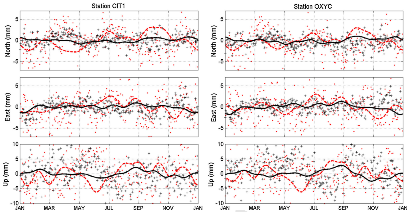
Fig. 10 Effect of periodic pattern of first reprocessing ( red ) and second reprocessing ( black ) campaign estimated for a typical example in which stations are close to each other. CIT1 is the site at California Institute of Technology. OXYC is the site at Occidental College. OXYC and CIT1 are 7 Km apart. The red and black points denote the residual time series
