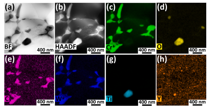
Fig. 8. STEM images of the ODS aged sample. (a) BF image, (b) HAADF image, (c) Cr (K) map, (d) O (K) map, (e) C (K) map, (f) W (M) map, (g) Ti (K) map and (h) Y (L) map.
