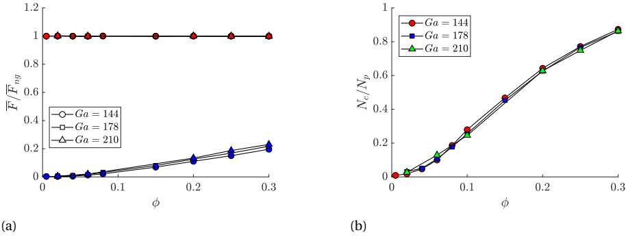
Figure 3.13: ((a)) Mean vertical drag force ( \bar{F}_d , red symbols) and mean magnitude of the collision force ( |\bar{F}_c| , blue symbols) normalised with the net gravity force ( \bar{F}_{ng} ) and shown as function of \phi and Ga . Circles, squares and triangles correspond to Ga = 144 , 178 and 210, respectively. ((b)) Average number of particles undergoing a collision during a computational time step ( N_c ), scaled with the total number of particles ( N_p ) and shown as function of \phi and Ga .
