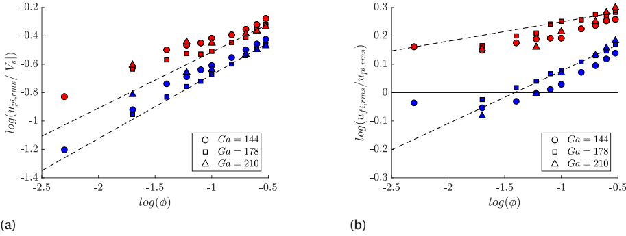
Figure 3.7: Double-log plot of ((a)) the particle rms velocity normalised with |V_s| and ((b)) the fluid/particle rms velocity ratio as function of \phi and for the three different Galileo numbers. Red and blue symbols refer to the vertical ( y ) and lateral ( x and z ) direction, respectively. Circles, squares and triangles correspond to Ga = 144 , 178 and 210, respectively. The dashed lines represent power-law fits of the DNS data to Eq. (3.6a) and (3.6b) for Ga = 178 and \phi \geq 10\% .
