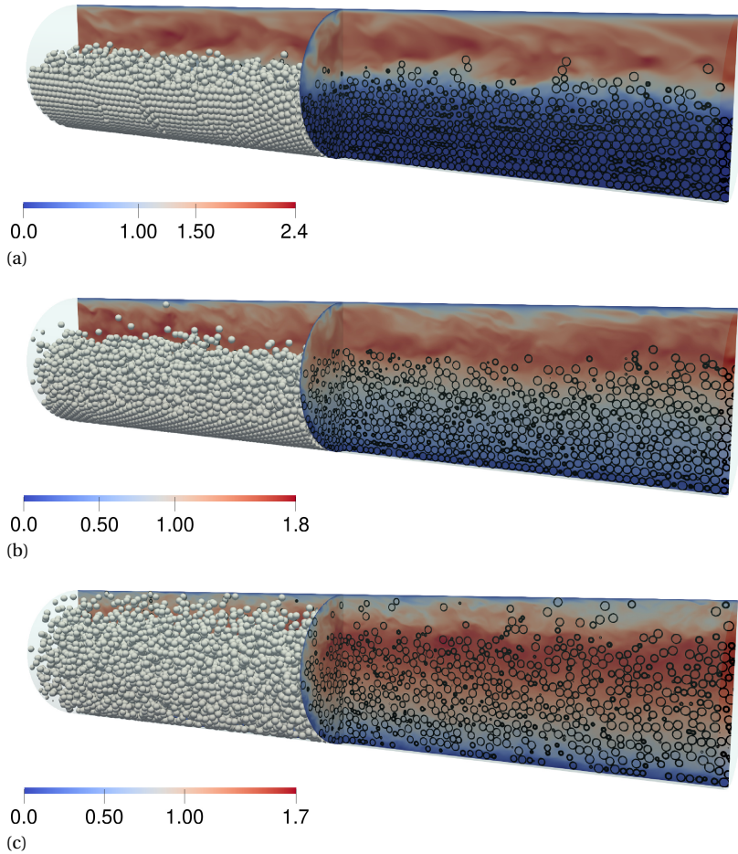
Figure 4.4: Instantaneous flow snapshots from the DNS in an xz and the yz plane along the pipe axis. The flow is going from left to right. The color denotes the streamwise velocity normalised with the liquid bulk velocity. Contours indicate the particle positions (local grid cell solid volume fraction equal to 0.5). The 3D spatial particle distribution is shown for part of the pipe in grey color. (a) D1, (b) D2, and (c) D3.
