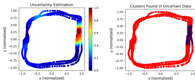
(a) Estimated aleatoric uncertainty of the data. The color of complete database and points the data indicates the uncertainty in the computed at each point. (b) Points in red represent the complete database and points the data belong to the detected cluster.
