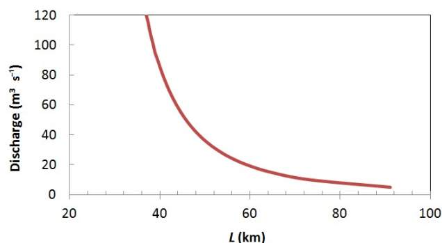
Figure 10. Relationship between river discharge and predicted salt intrusion length.
