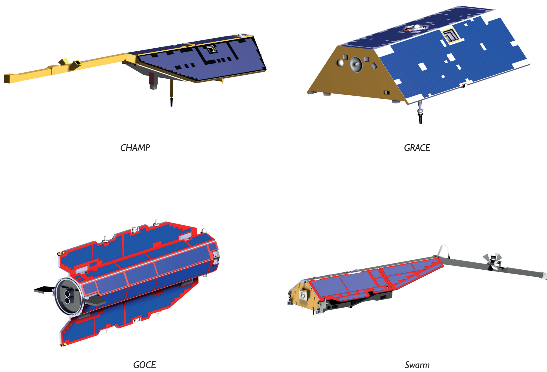
Satellite geometry models designed with CATIA V5 R21.
