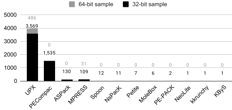
Fig. 6. Identified packers from the virus dataset.
