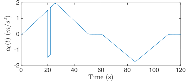
Fig. 3. Desired platoon acceleration a_0(t) .
