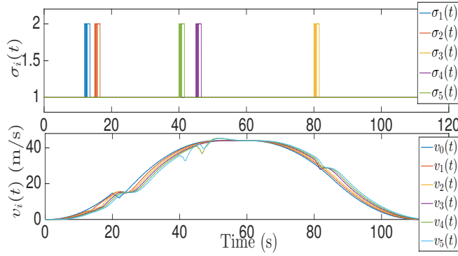
Fig. 5. Experiment 3: Switching signals \sigma_i(t) of vehicles 1-5: \sigma_i(t) , i \in S_5 (Top) and Velocities of vehicles 0-5: v_i(t) , i \in \{0, 5\} (Bottom).
