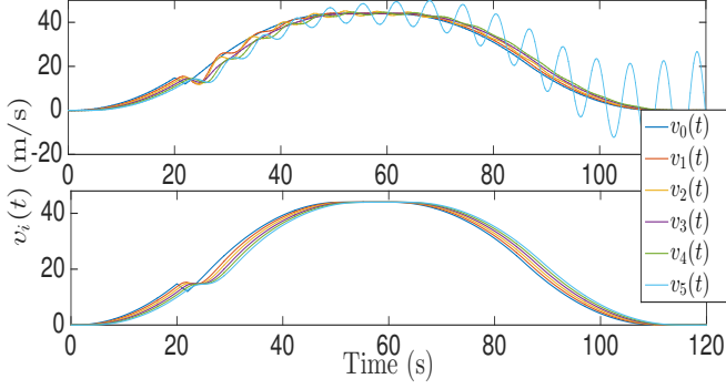
Fig. 4. Velocities of vehicles 0-5: v_i(t) , i \in \{0, 5\} in Experiment 1 (Top) and Experiment 2 (Bottom).
