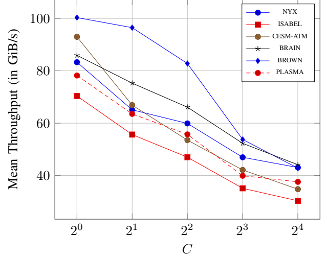
Figure 7: GPU decoding throughput, under Strategy 1, as a function of C
