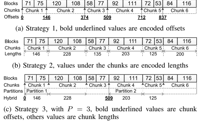
Figure 2: Metadata under different strategies for 12 blocks of the Brain benchmark [12] that was compressed using ZFP with a fixed accuracy of 0.05. For all strategies we used C = 2 , values inside the blocks are the block lengths in bits
