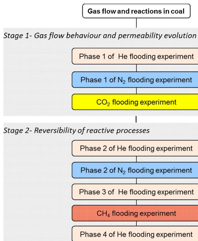
Fig. 1. The flow diagram of the experimental studies on gas flow behaviour in coal and permeability evolution.
