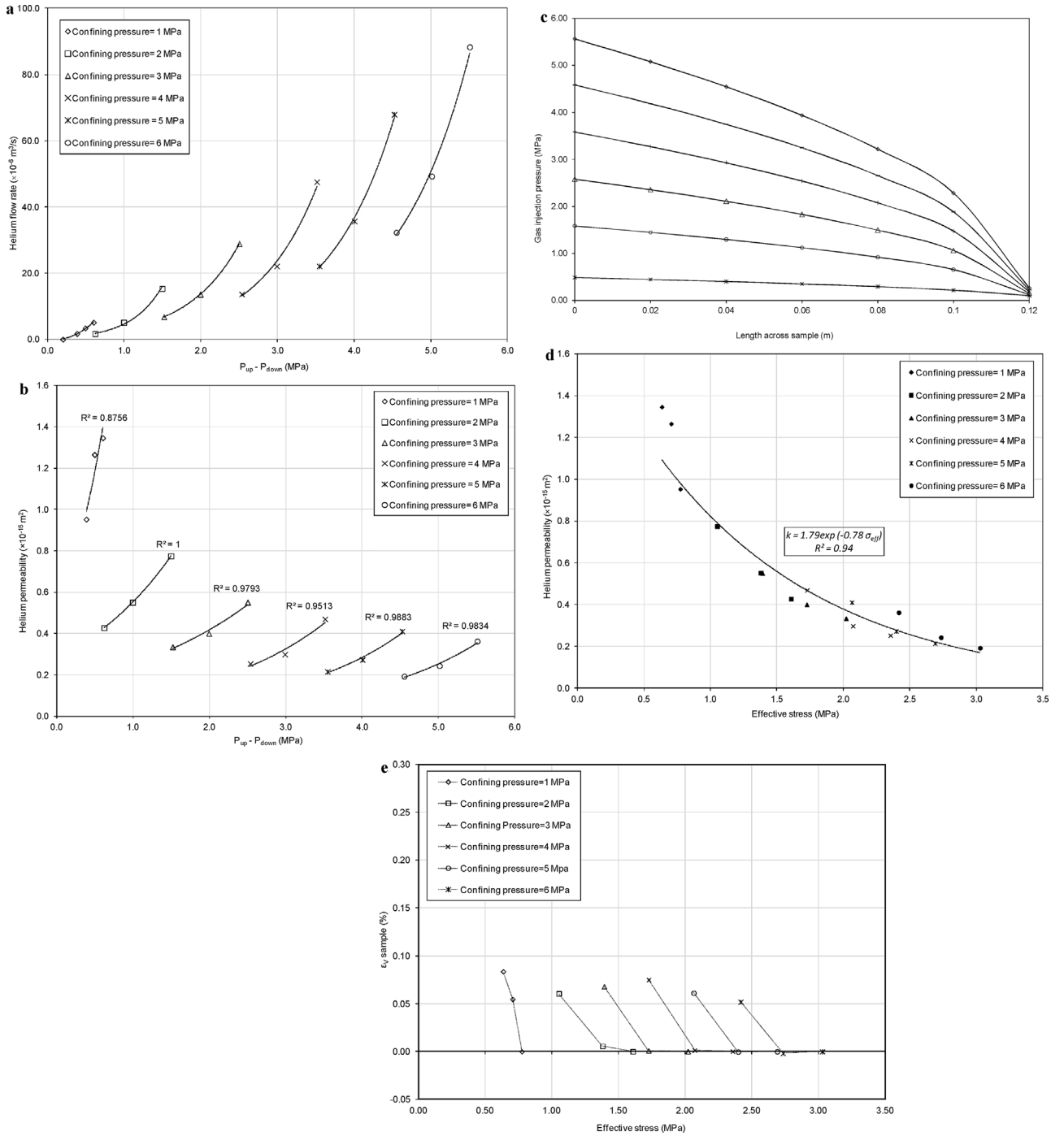
Fig. 4. (a) Variations of helium flow rates versus differential gas pressure between the upstream and downstream at various confining pressures ( T = 298 \text{ K} ). (b) Variations of absolute permeability of the coal sample to helium versus differential gas pressure between upstream and downstream at various confining pressures ( T = 298 \text{ K} ). (c) Variation of gas pore pressure across sample length. (d) The relationship between coal permeability to helium and effective stress ( T = 298 \text{ K} ). (e) Variations of the volumetric expansion of the coal sample versus effective stress due to the increase in helium pressure at constant confining pressures ( T = 298 \text{ K} ).
