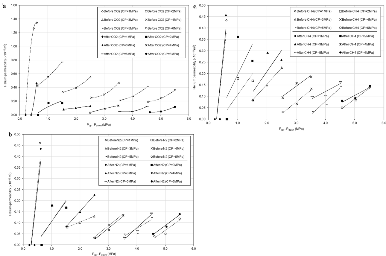
Fig. 7. (a) Variations of the helium permeability of the coal sample with differential gas pressure before (dashed line) and after (solid line) \text{CO}_2 injections ( T = 298 \text{ K} ). (b) Variations of the helium permeability of the coal sample with differential gas pressure before (dashed line) and after (solid line) the phase 2 of \text{N}_2 injections ( T = 298 \text{ K} ). (c) Variations of the helium permeability of the coal sample with differential gas pressure before (dashed line) and after (solid line) the \text{CH}_4 injections ( T = 298 \text{ K} ).
