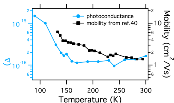
Figure 3. Maximum observed values of the photoconductance corrected for the incident number of photons ( I_0 = 2.8 \times 10^{12}/\text{cm}^2 ) and sample area versus temperature. Left and right axes both cover 2 orders of magnitude to allow comparison. The excitation wavelength is 500 nm. The temperature-dependent mobility values measured by PR-TRMC are imported from the paper of Gélvez-Rueda et al. 40
