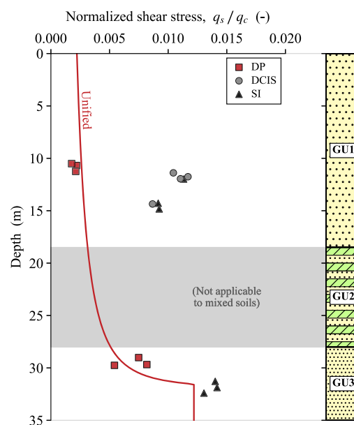
Fig. 14. Normalized peak shear stress of all piles in GU1 and GU3, including residual load in the DP piles.
