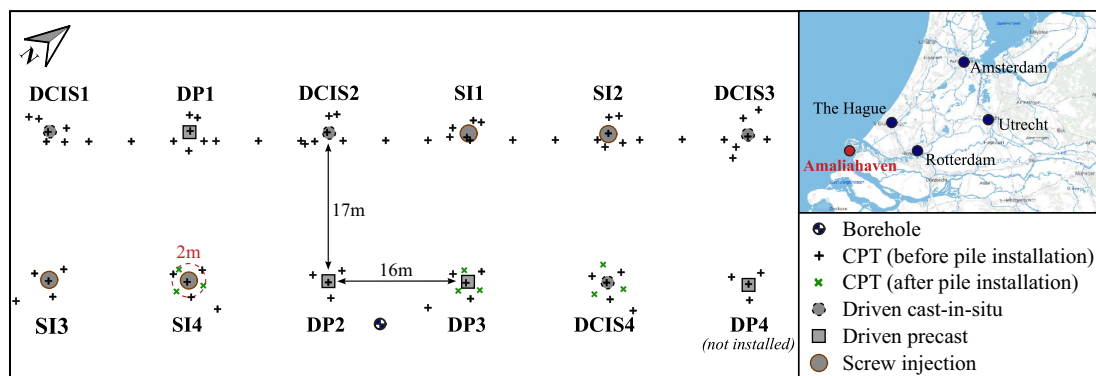
Fig. 1. Layout and location of the Amaliahaven test site. [Map courtesy of PDOK, under Creative Commons-BY-4.0 license ( https://creativecommons.org/licenses/by/4.0/ ).]
