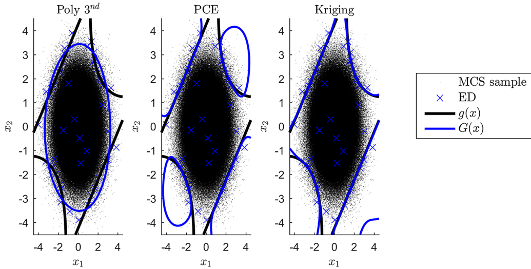
Fig. 10. Example of surrogate approximation given by higher-order models considered in the basis, the 3 nd polynomials, PCE and Kriging, for an ED (49 points) obtained with the complement-basis and the proposed active learning implementation.
