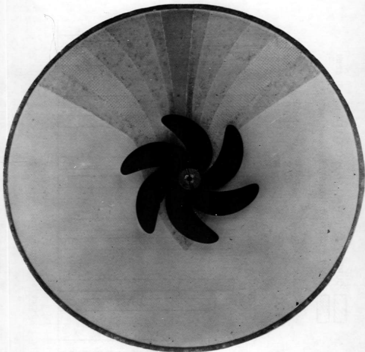
Figure 17 – Wake Screen and Highly Skewed Model Propeller 4452
