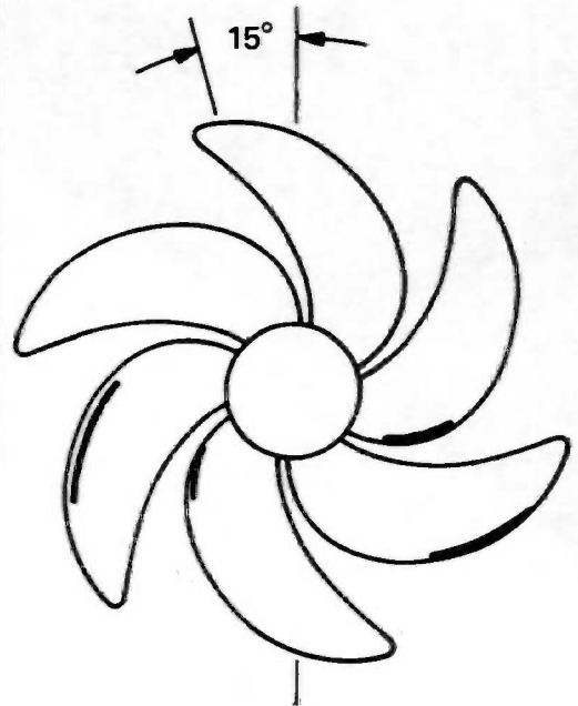
Figure 21 – Cavitation at 26 Knots
