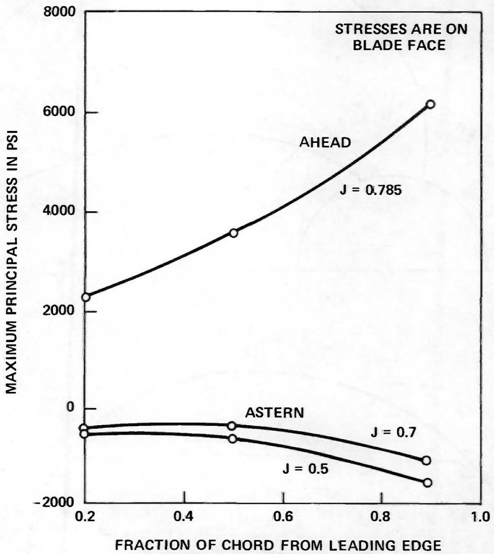
Figure 24 - Principal Stresses
