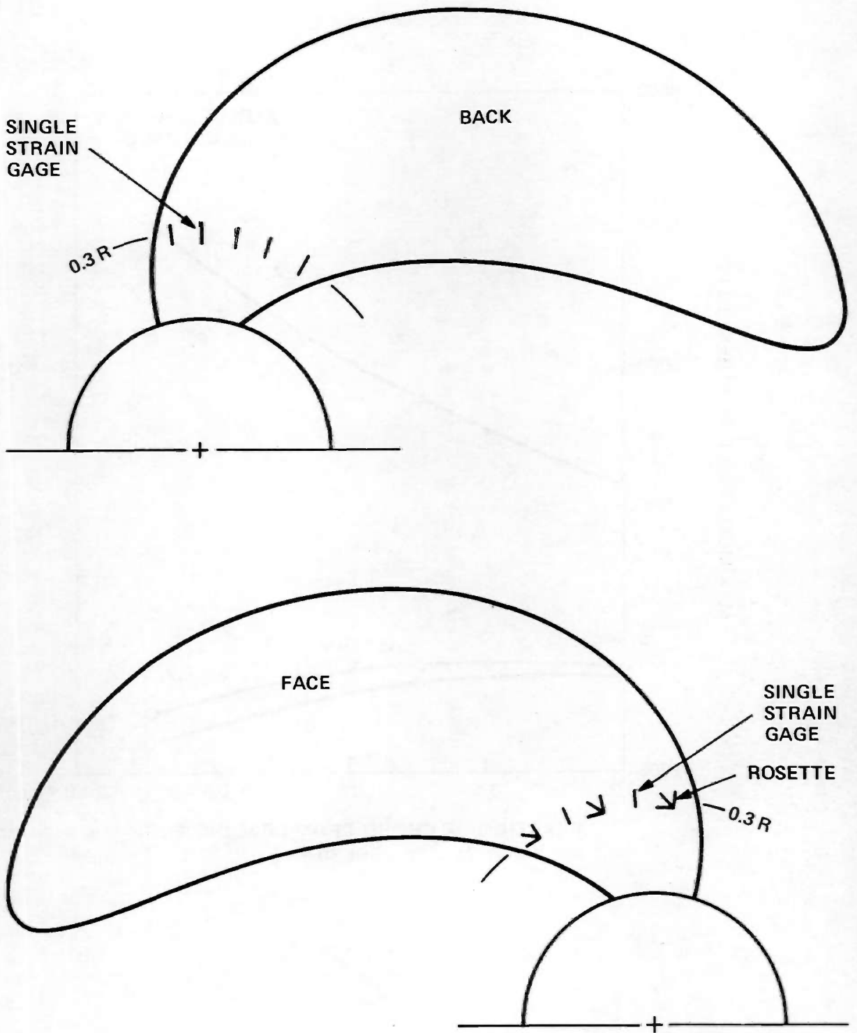
Figure 23 – Location of Strain Gages and Rosettes
