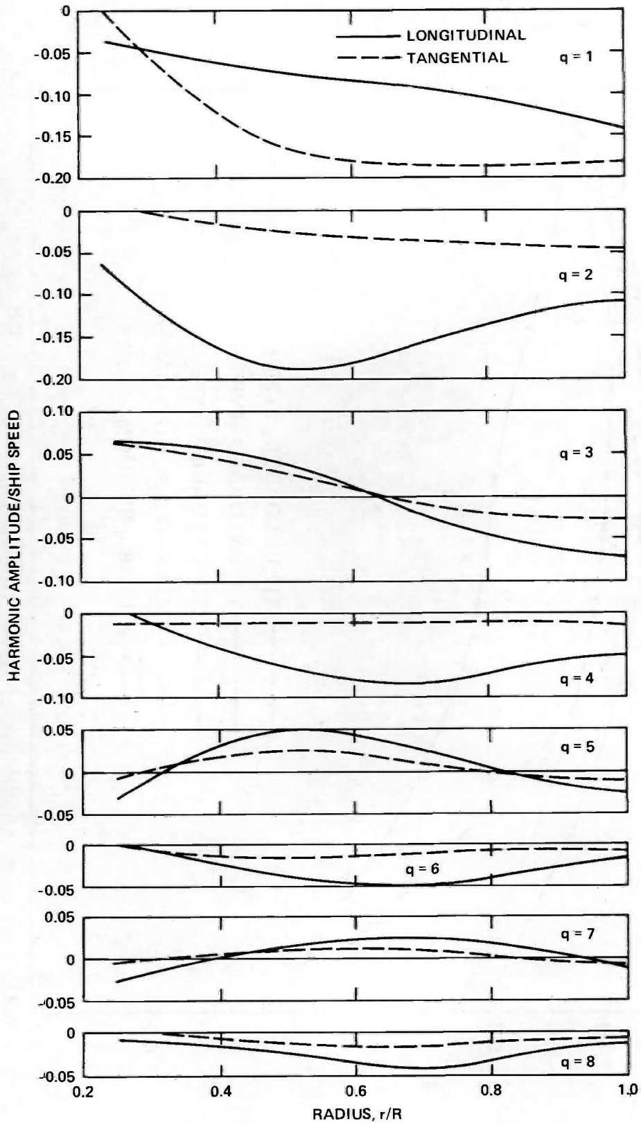
Figure 3 – Harmonic Amplitudes of Wake Velocities
