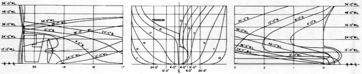
Figure 1 - Hull Lines
