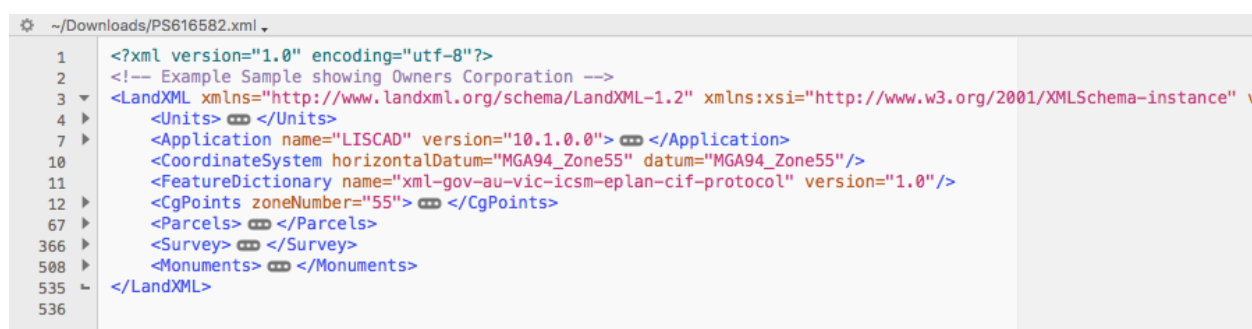
Figure 3. Structure of an ePlan compliant LandXML file
