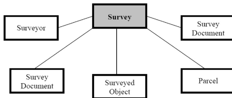
Figure 2. Overview of the ePlan data model diagram (Karki et al., 2011)
