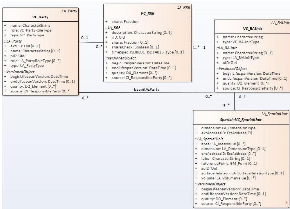
Figure 55. The four fundamental classes of the Victoria LADM-based country profile
