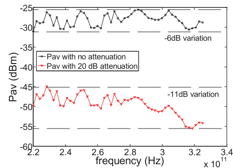
Fig. 2 - Variation of the measurement dynamic range across the frequency band due to the limited flatness of the frequency response and the use of the attenuator [5].
