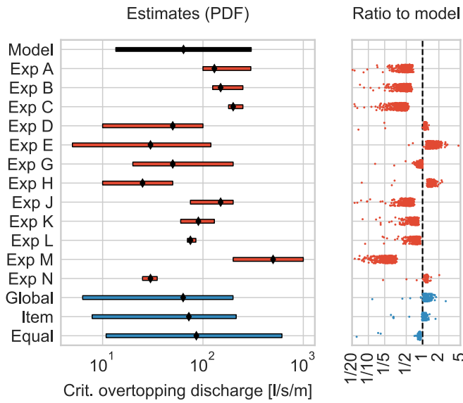
Fig. 8. Experts' estimates for the critical overtopping discharge that causes a breach when exposed for a 6-hour duration. The model result is derived from the log-normal distribution for H_s in [0 - 1] m and an open grass quality. Because of the log-scale, the bar heights are not scaled to the probability density. The ratios on the right are shown as scatters, with each dot representing the ratio for a single dike section.
