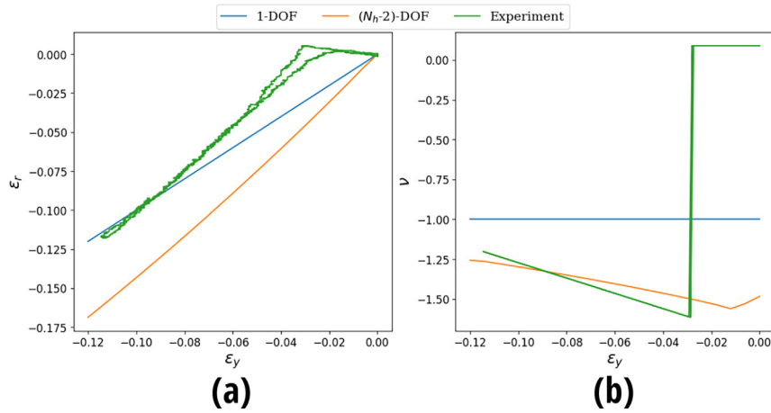
Figure 6. Plots of (a) radial strain and (b) ratio as a function of the applied vertical strain on the structures. Shown are the data from the experiment (green), and the calculated values for the one-degree-of-freedom (blue) and (N_h - 2) -degrees-of-freedom (orange) pseudo-rigid body model. DOF: degree(s) of freedom.
