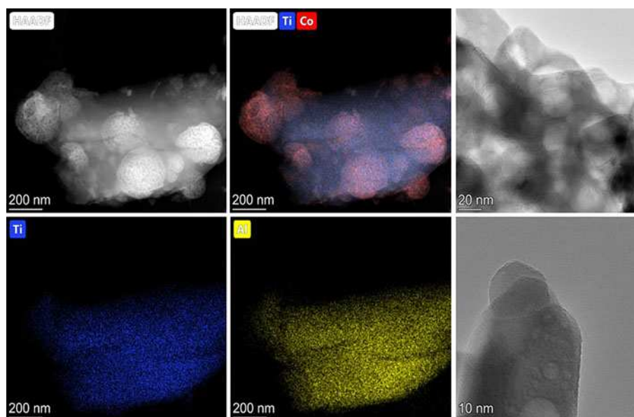
Figure 3. HAADF-STEM images of \text{Co}_3\text{O}_4/\text{Ti}_2\text{AlC} catalyst.
