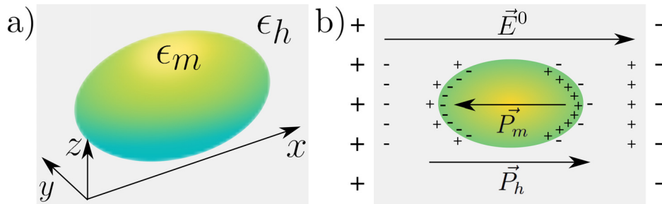
Fig. 3. (a) Ellipsoidal particle immersed in a dielectric medium with the chosen reference system. (b) Snapshot of the incoming electric field and the induced polarization contributions of the metal and the host. This depiction is realistic only in the optical regime and under the quasi-static approximation (QSA), for which the rearrangement of charge is collective and instantaneous.
