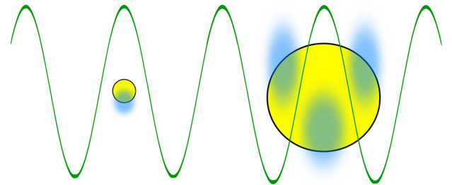
Fig. 2. Dipolar (left) and multipolar (right) excitation of the free electrons in metal nanoparticles. The electron clouds are represented as light blue halos, while the metal cores as solid yellow.
