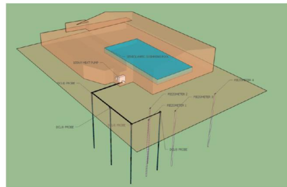
Figure 5: Scheme showing the wells positioning at the public swimming pool in Nules, in black: DCL probes, in red: monitoring wells.
