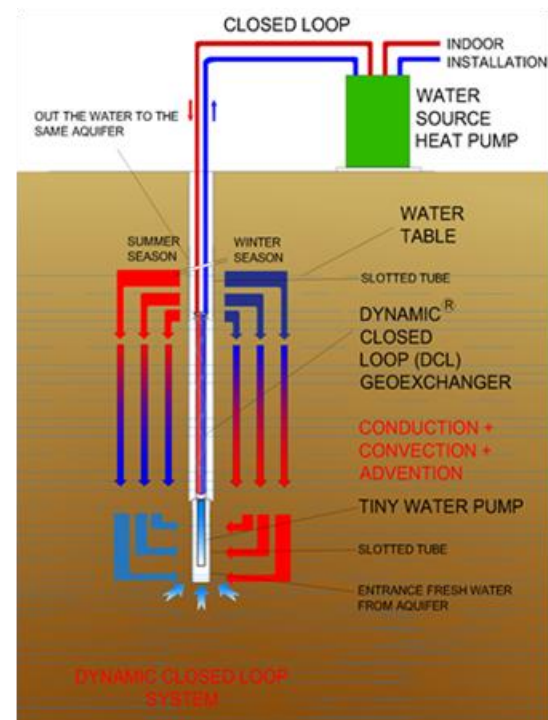
Figure 4: Scheme of the DCL® probe system tested in the Spanish pilot site.
