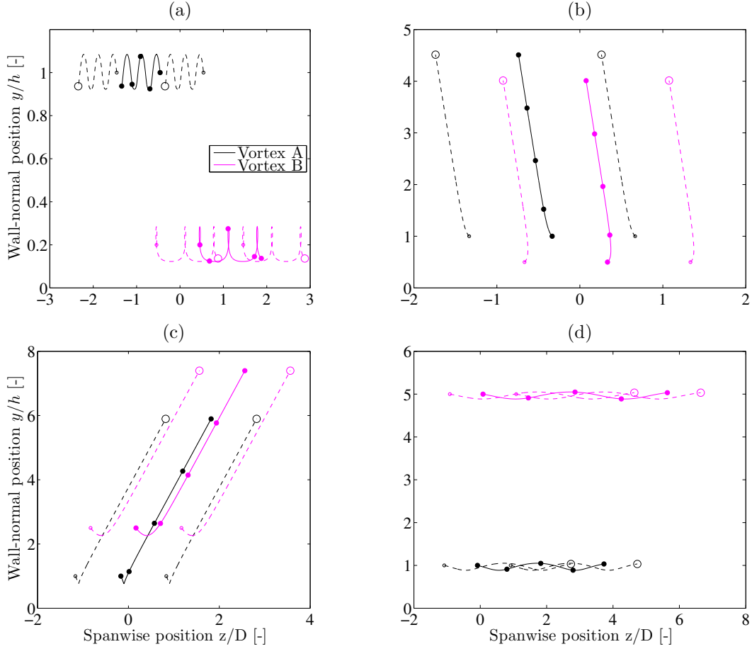
Figure 5: Trajectories for \Gamma = -1 , for different initial conditions (\Delta z_0/D, \Delta y_0/h) : (a) 11/12, -0.8; (b) 2/3, -0.5; (c) 1/3, 1.5 and (d) 1/6, 4.0. Filled markers and solid lines represent the base vortices; empty markers and dashed lines represent their periodic images. Markers are spaced at 0.25\mathcal{T} . Trajectories (a) and (b) are shown for a total time 1L/U , (c) for 5L/U and (d) 10L/U .
