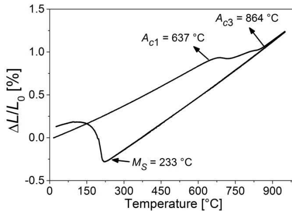
Figure 5.7 Dilatation versus temperature during heating at 3 K/min to 950\text{ }^{\circ}\text{C} , holding and cooling. The A_{c1} -, A_{c3} - and M_s -temperatures are indicated.
