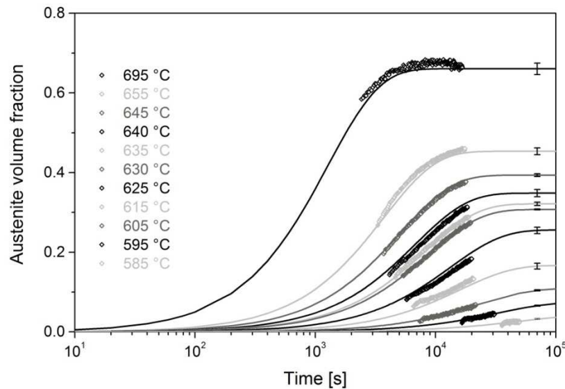
Figure 6.16 Solid lines give the volume fraction of austenite at T_{1t} as a function of time obtained by equation (6.4). The symbols show the experimental data. The error bars, drawn at a time of 7 \cdot 10^4 \text{ s} , show the standard error for the austenite fraction f_{\gamma} obtained by equation (6.4). The tempering temperatures T_{1t} are indicated.
