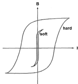
Figure 2.16 Comparison of characteristic magnetization curves of “soft-” and “hard-magnetic” materials [49].
