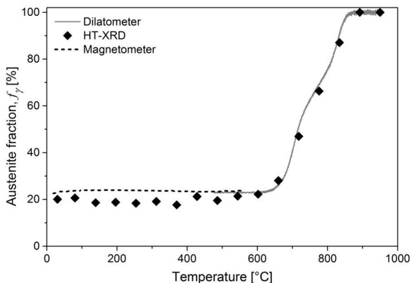
Figure 5.5 Austenite fraction, f_\gamma , of as-received 13Cr6Ni2Mo SMSS during heating obtained from thermo-magnetic measurement, dilatometry and HT-XRD experiment.
