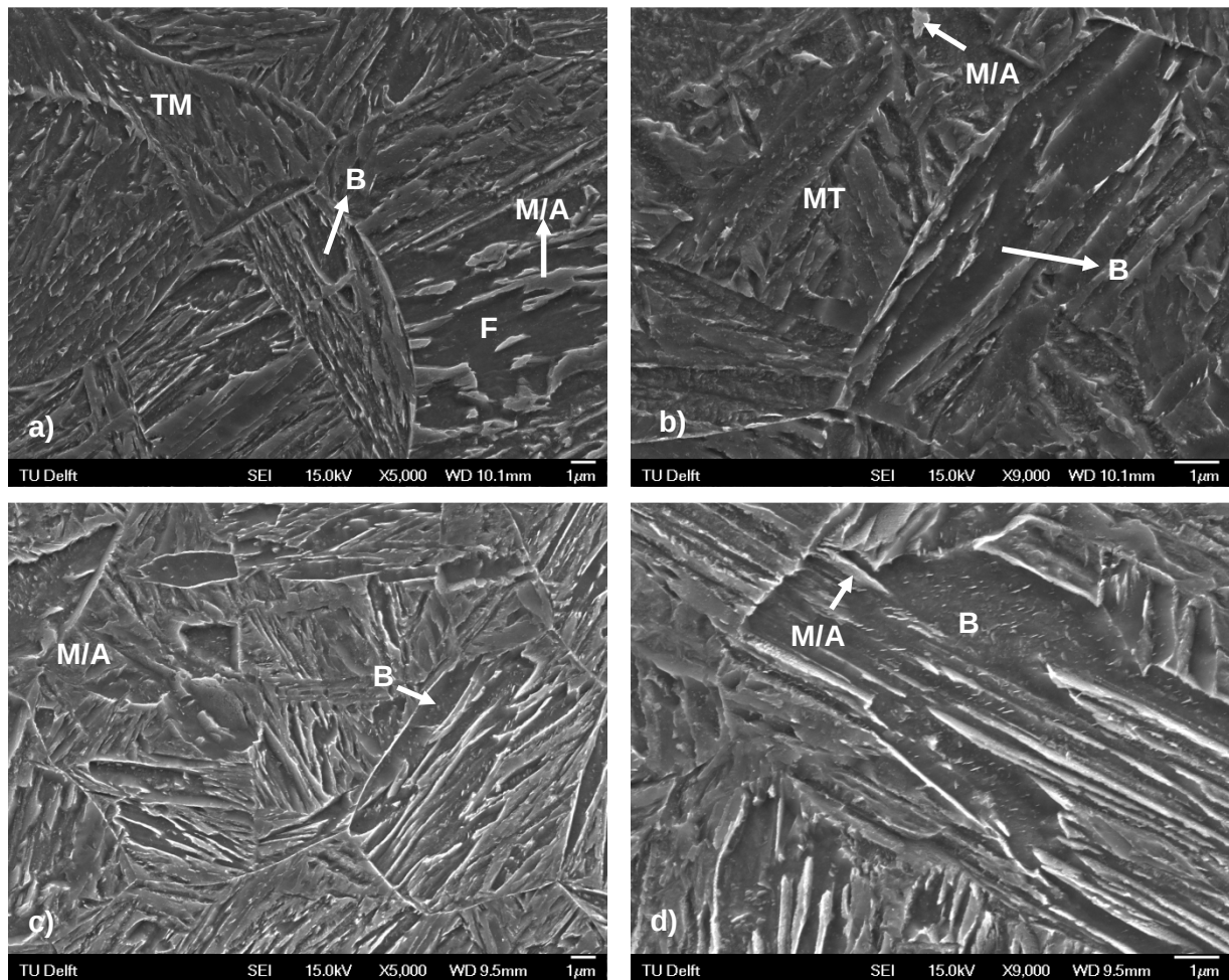
Figure 8.18 Microstructure of steel 0.2C. a)-b) Experiment in VSM with cooling from 906 °C, \tau = 38 min. c)-d) Experiment in dilatometer with cooling from 900 °C, \tau = 20 min. M denotes martensite, TM tempered martensite, A austenite, F ferrite and B bainite.
