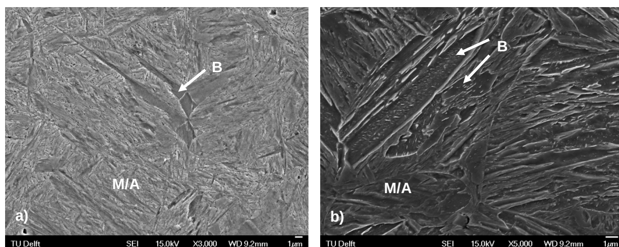
Figure 8.4 Microstructures of the as-received steels. a) 0.6C-steel b) 0.2C-steel. M denotes martensite, A austenite and B bainite.
