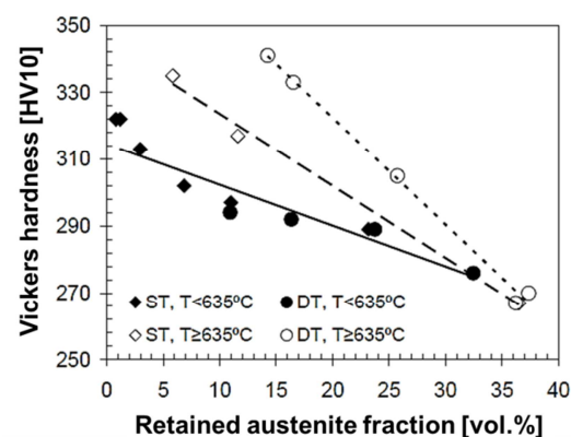
Figure 2.12 Effect of retained austenite fraction on hardness of a 13Cr6Ni2Mo SMSS after single tempering (ST) and double tempering (DT) (modified from [9]). ST for 4 h, DT at 550 °C for 2 h. T_{peak} = 635 °C.
