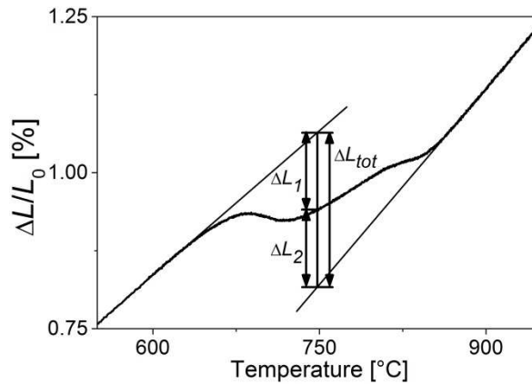
Figure 3.13 Example of a dilatation curve of an as-received 13Cr6Ni2Mo SMSS sample during heating. The parameters for determining the transformed fraction from the dilatation by the lever rule are indicated. \Delta L/\Delta L_0 is the length change normalized by the initial sample length. \Delta L_1 denotes the difference between the measured length change and the extrapolated length change of the transformed phases, \Delta L_2 the difference between the measured length change and the extrapolated length change of austenite and \Delta L_{tot} the total length change, all at a specific temperature.
