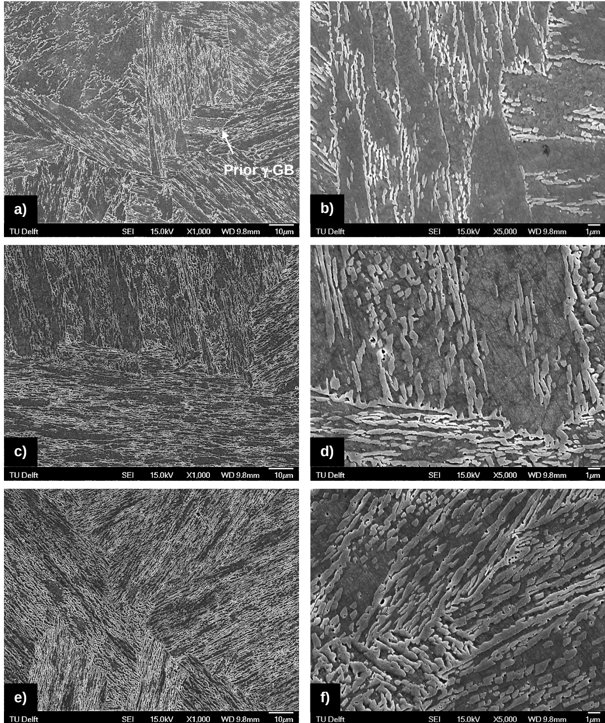
Figure 6.12 SEM micrographs after single tempering for 4 h at a),b) 615 °C, c),d) 635 °C and e),f) 655 °C. Dark grey areas: tempered martensite, light grey areas: retained austenite ( T_{1t} \leq T_{peak} ) and retained austenite + fresh martensite [4] ( T_{1t} > T_{peak} ). Prior \gamma GB: prior austenite grain boundary.
