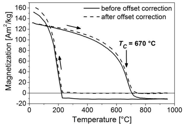
Figure 3.9 Magnetization versus temperature of an as-received 13Cr6Ni2Mo SMSS sample during heating to 950 °C and cooling. Heating and cooling are indicated by arrows. The Curie temperature, T_C is indicated.
