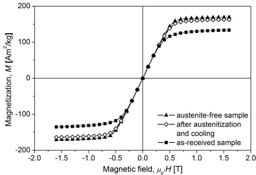
Figure 5.2 Room temperature curve of magnetization M versus the magnetic field ( \mu_0 \cdot H ) for the as-received sample, the austenitized sample and the austenite-free sample.
