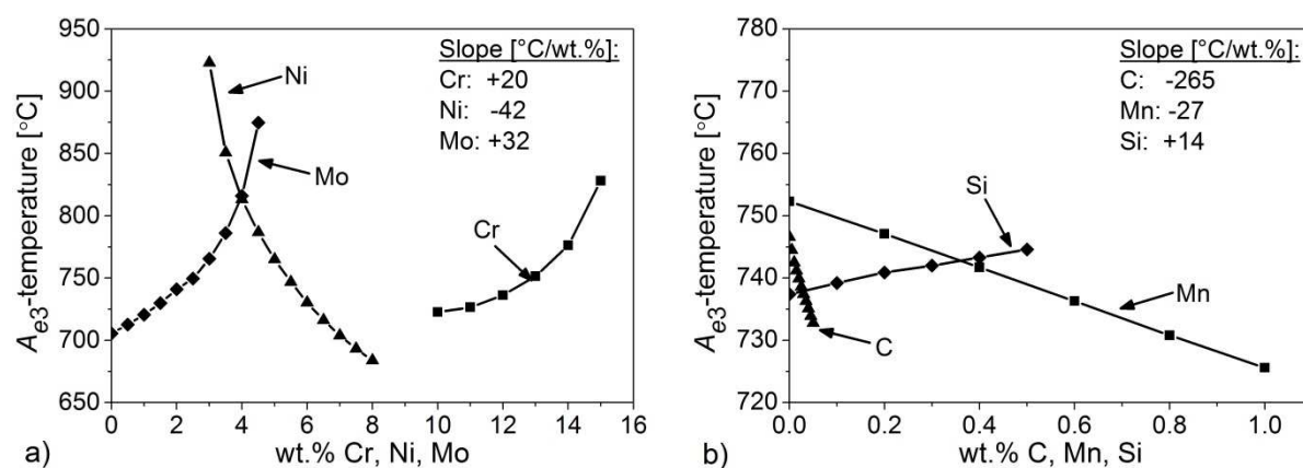
Figure 4.3 Influence of the variation of the main alloying elements on the A_{e3} -temperature of the 13Cr6Ni2Mo SMSS balanced with Fe. The average slopes of the curves are indicated.
