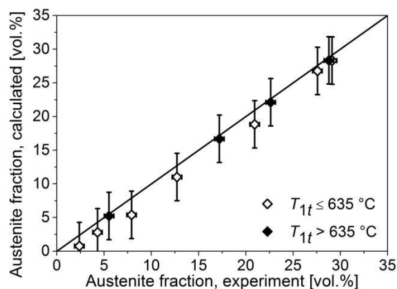
Figure 6.21 Calculated austenite fraction (see Figure 6.20) versus the austenite fraction obtained after cooling from the first tempering temperature and holding at room temperature until the values became stable.
