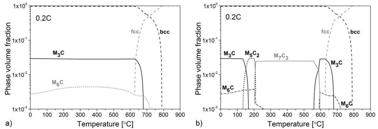
Figure 8.6 Equilibrium phase fractions obtained by Thermo-Calc [16] for steel 0.2C. a) Only carbides present for calculations: cementite and M_6C . b) Several carbides allowed to be present for calculations. M = Fe and Mn in M_3C , M_5C_2 , M_7C_3 , and M = Mo and Fe in M_6C .
