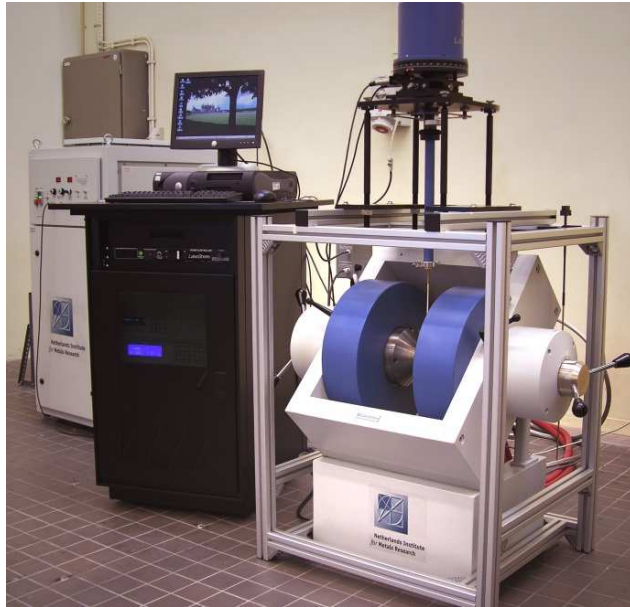
Figure 3.3 Lake Shore 7307 Vibrating Sample Magnetometer with room temperature set-up.
