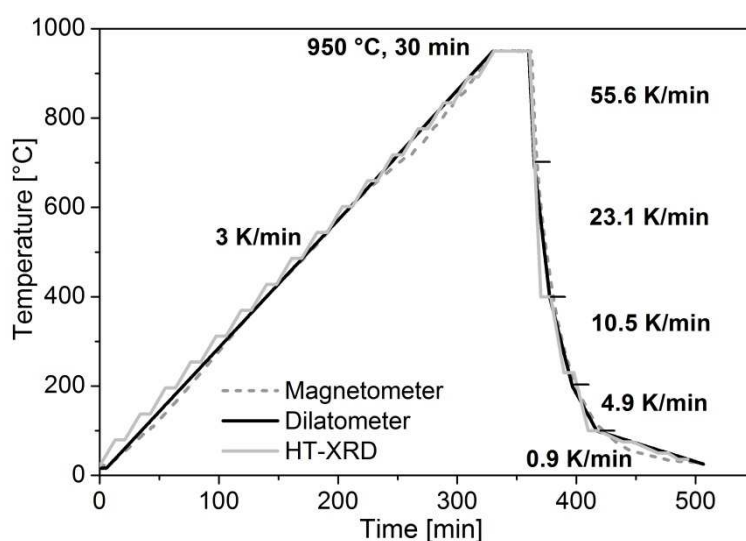
Figure 5.1 Temperature-time profiles for thermo-magnetic, dilatometer and HT-XRD experiments. The cooling rates indicated in the figure are for the dilatometer experiment.
