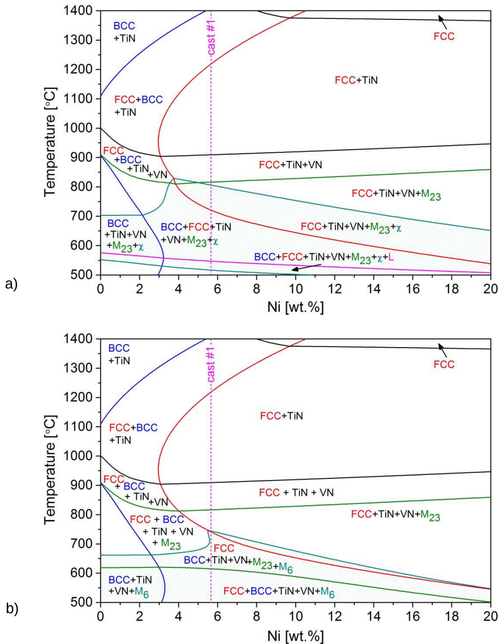
Figure 4.5 Pseudo-binary phase diagrams for 13Cr6Ni2Mo SMSS, cast #1. a) \chi - and Laves (L)-phases present. b) \chi - and Laves-phases absent. The blue line indicates the presence of bcc-ferrite and the red line the presence of the fcc-austenite single phase field, without consideration of carbides and nitrides, \chi - and Laves-phases. The dotted magenta line indicates the bulk Ni-content of cast #1. M 23 and M 6 represent M 23 C 6 and M 6 C. The hashed area indicates the presence of \chi -phase and M 6 C, respectively.
