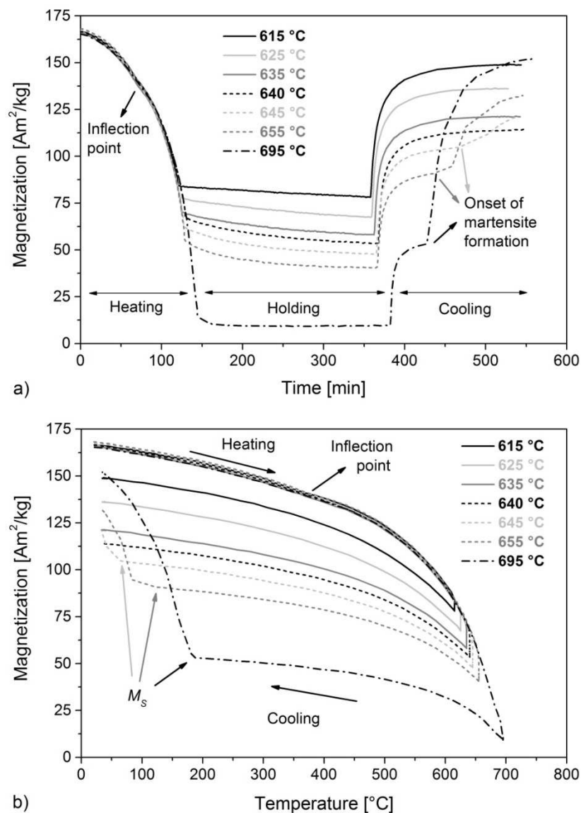
Figure 6.3 Magnetization versus a) time and versus b) temperature during the first tempering step, measured at a field of 1.5 T. The tempering temperatures T_{1t} are indicated.
