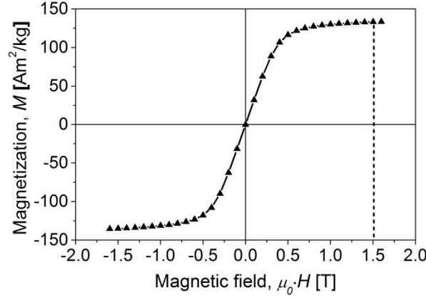
Figure 3.7 Room temperature curve of magnetization M versus the magnetic field ( \mu_0 H ) for the as-received 13Cr6Ni2Mo SMSS. The dashed line indicates the magnetic field of 1.5 T at which the magnetization was measured during the thermo-magnetic experiments.
