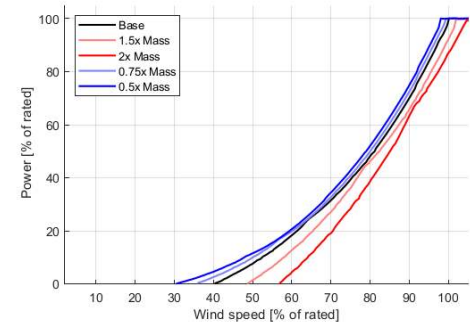
Figure 1: Power curves for a kite system at 5 different airborne masses normalised by the baseline system.
