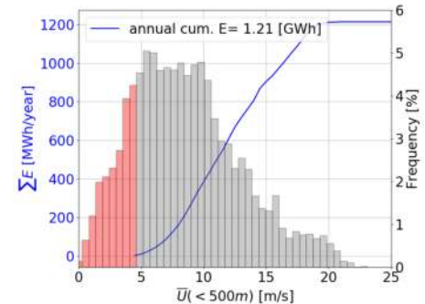
Estimated annual energy production of a 12 m 2 wing area ground-generation AWES (blue) over mean wind speeds up to 500 m. Wind inflow is based on 10-min onshore WRF model. The background shows the WRF-simulated annual probability distribution of average wind speeds up to 500 m.
