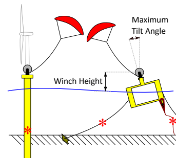
Key parameters for re-powering and floating AWE. Red * indicate locations of fatigue.
