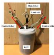
Figure 1: Kite power system: KCU, and Real Flight Test.
