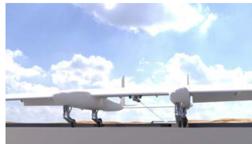
Tether-arrested landing, showing aircraft landing on a platform with tailored arresting system.
