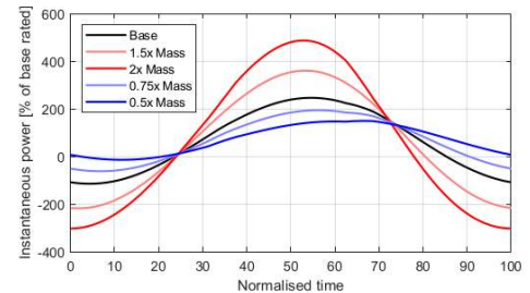
Figure 2: Variation in instantaneous power during a single circular flight trajectory for 5 different airborne masses at the nominal rated wind speed.
