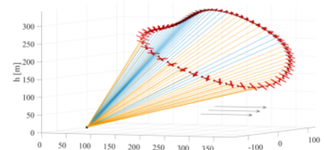
An optimal flight path for an airborne wind energy system to generate maximal power calculated by OpenOCL using CasADi and Ipopt , flight models from OpenAWE . The system generates power when the winch releases tether (indicated by the orange lines).
