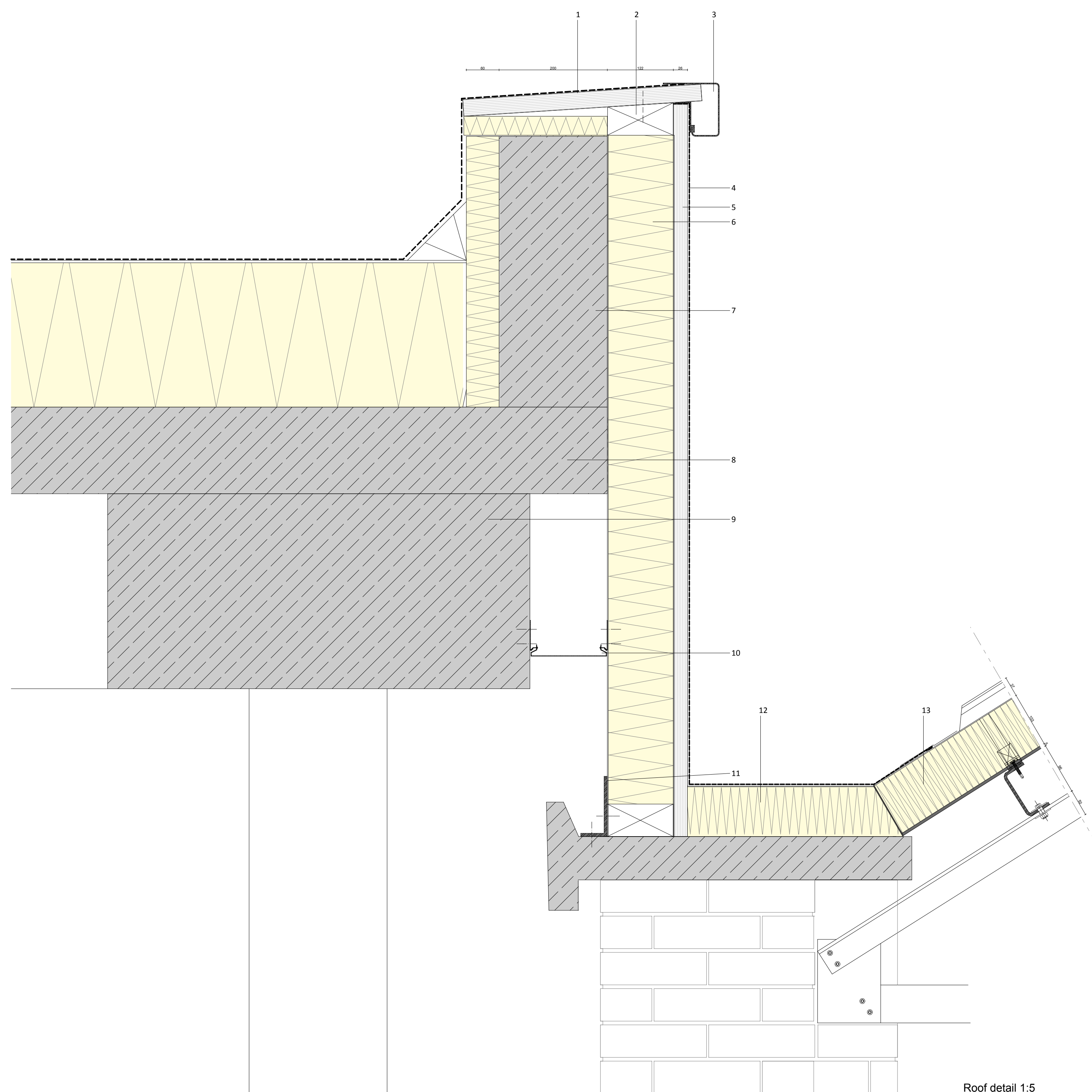
Roof detail 1-5
