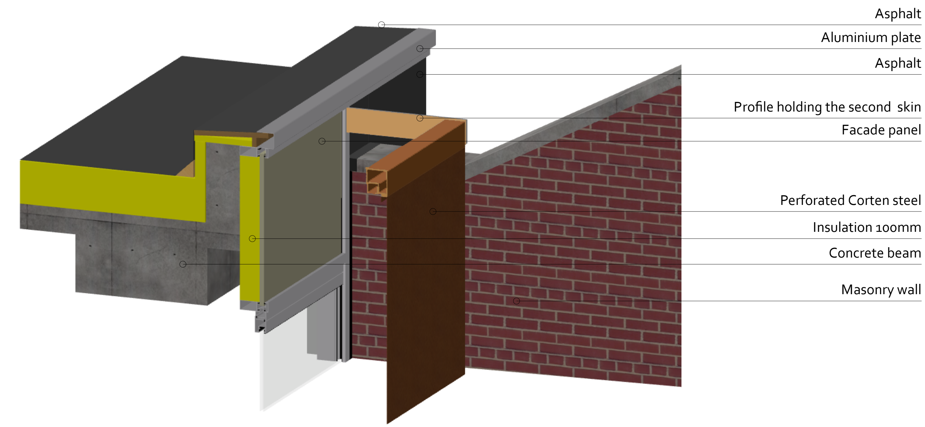
Roof detail 1
