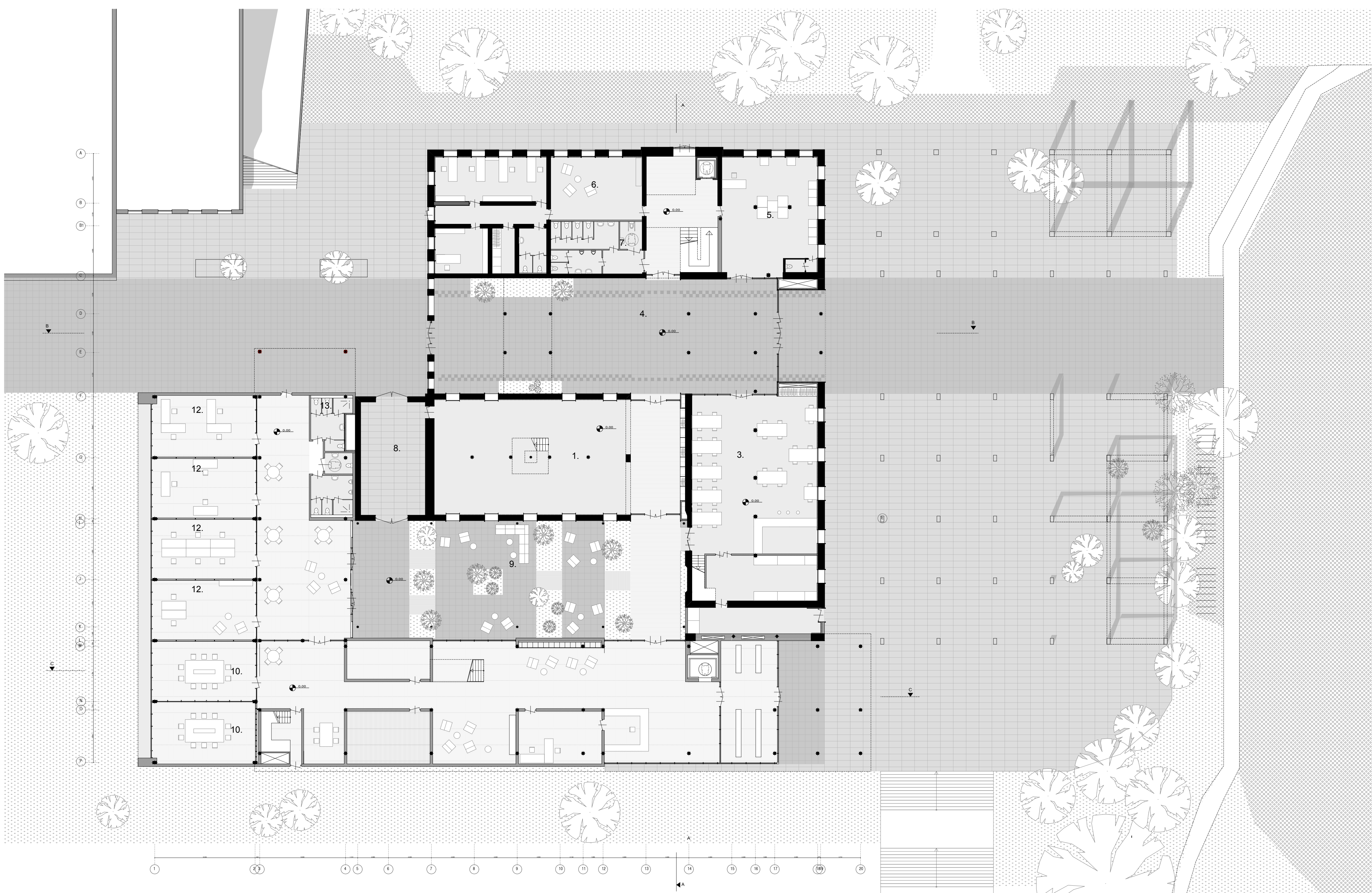
Ground floor 1:200
