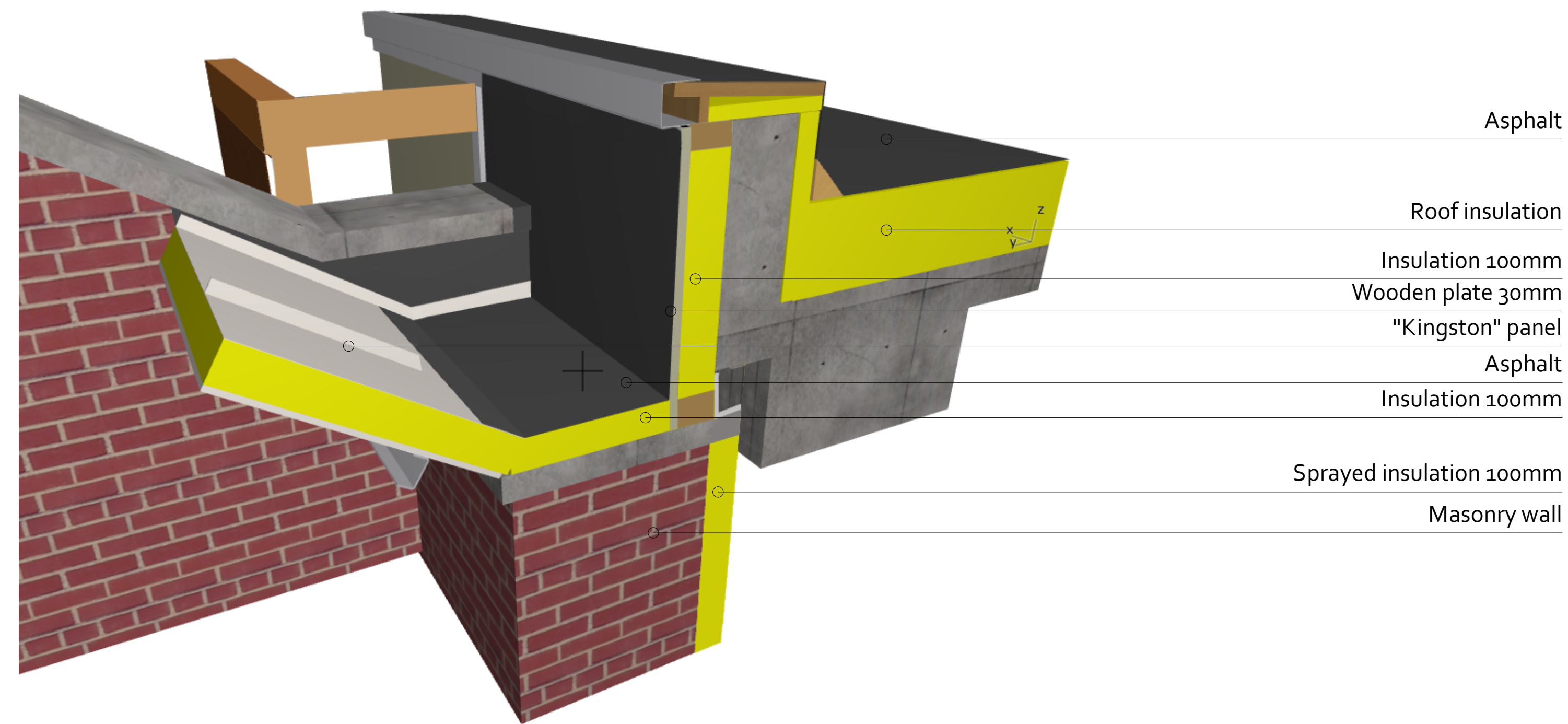
Roof detail 1
