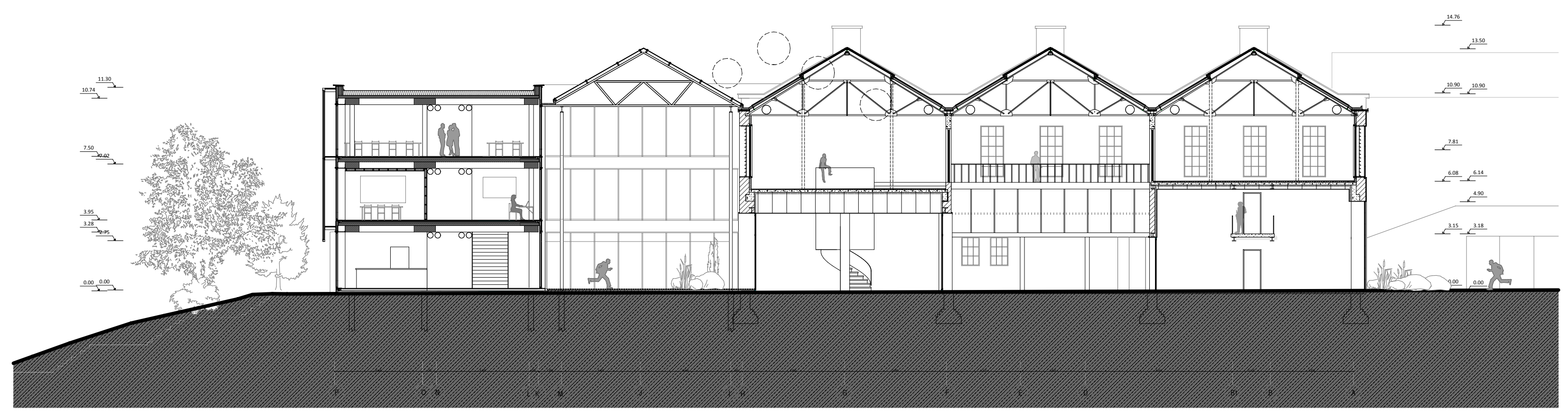
Building section 1:200
