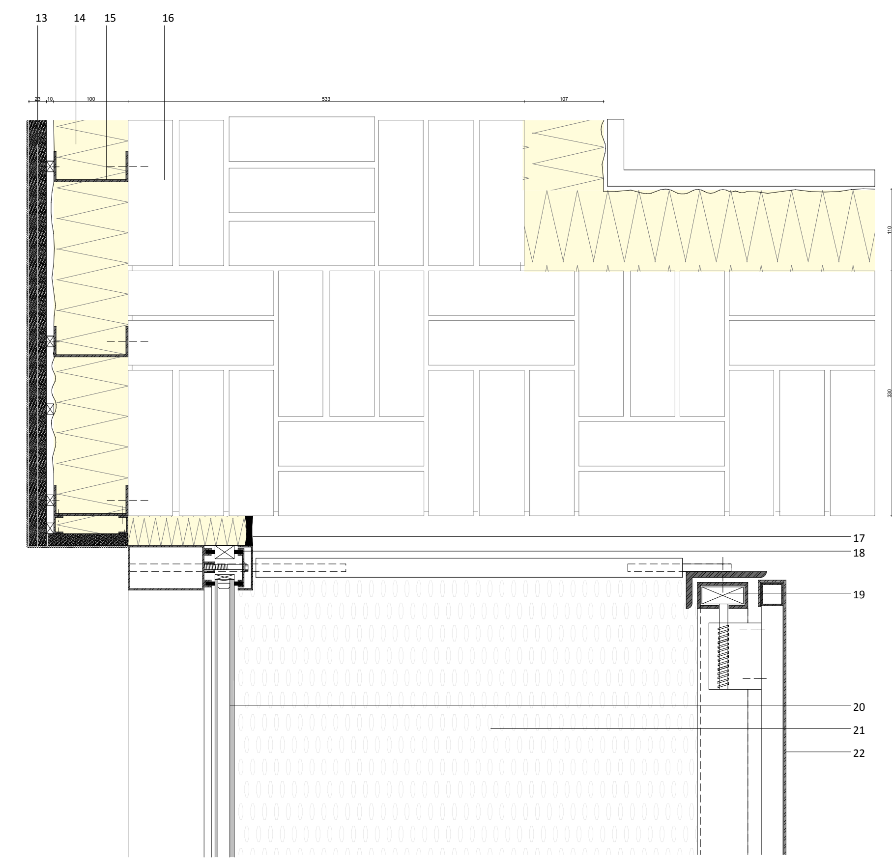
Horizontal roof detail 1-5
