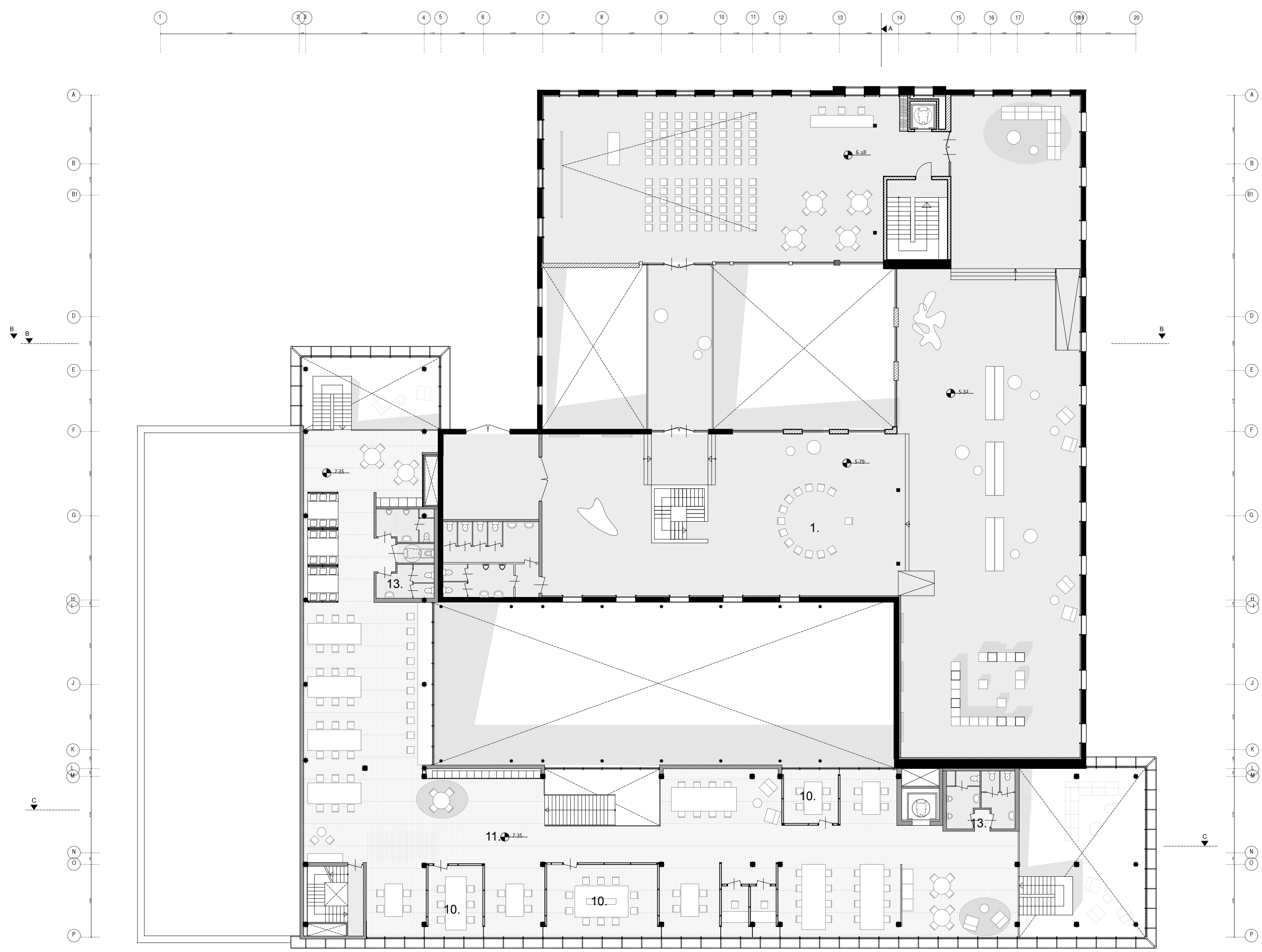
Second floor 1:200
