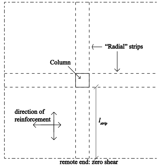
9 10 Figure 4 – Layout of quadrants and strips (Alexander and Simmonds, 1992). 11
