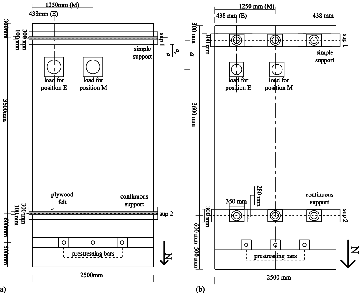
9 (a) (b) 10 Figure 2 – Test setup for slab shear experiments: (a) with line supports; (b) supported by elastomeric 11 bearings. Units: mm; 1 mm = 0.04 in. 12
