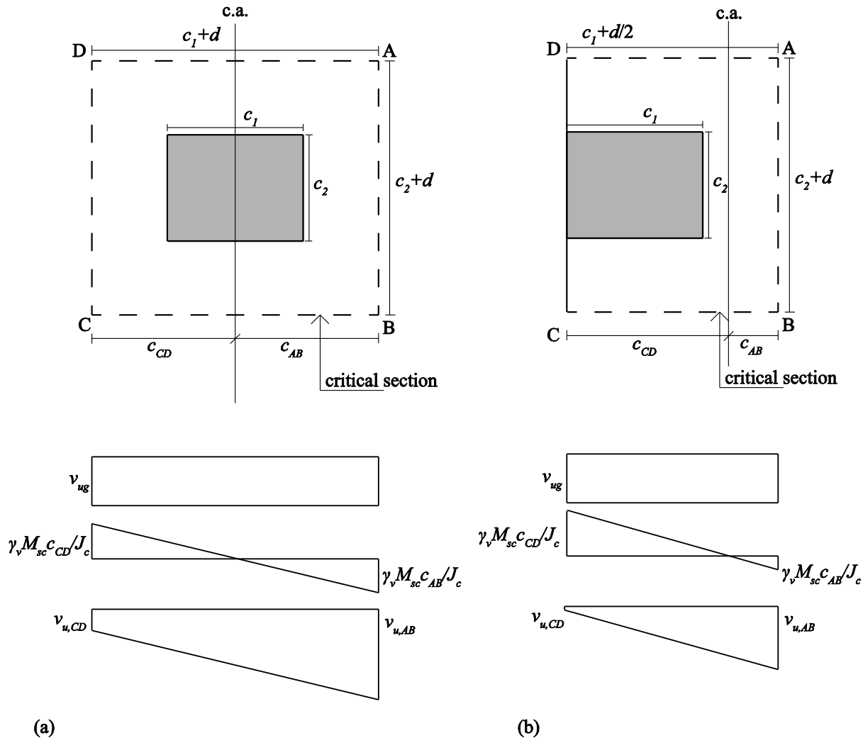
11 (a) (b) 12 Figure 1 – Determination of governing factored shear stress from the combination of direct shear and 13 unbalanced moments: (a) for an interior column; (b) for an edge column.
