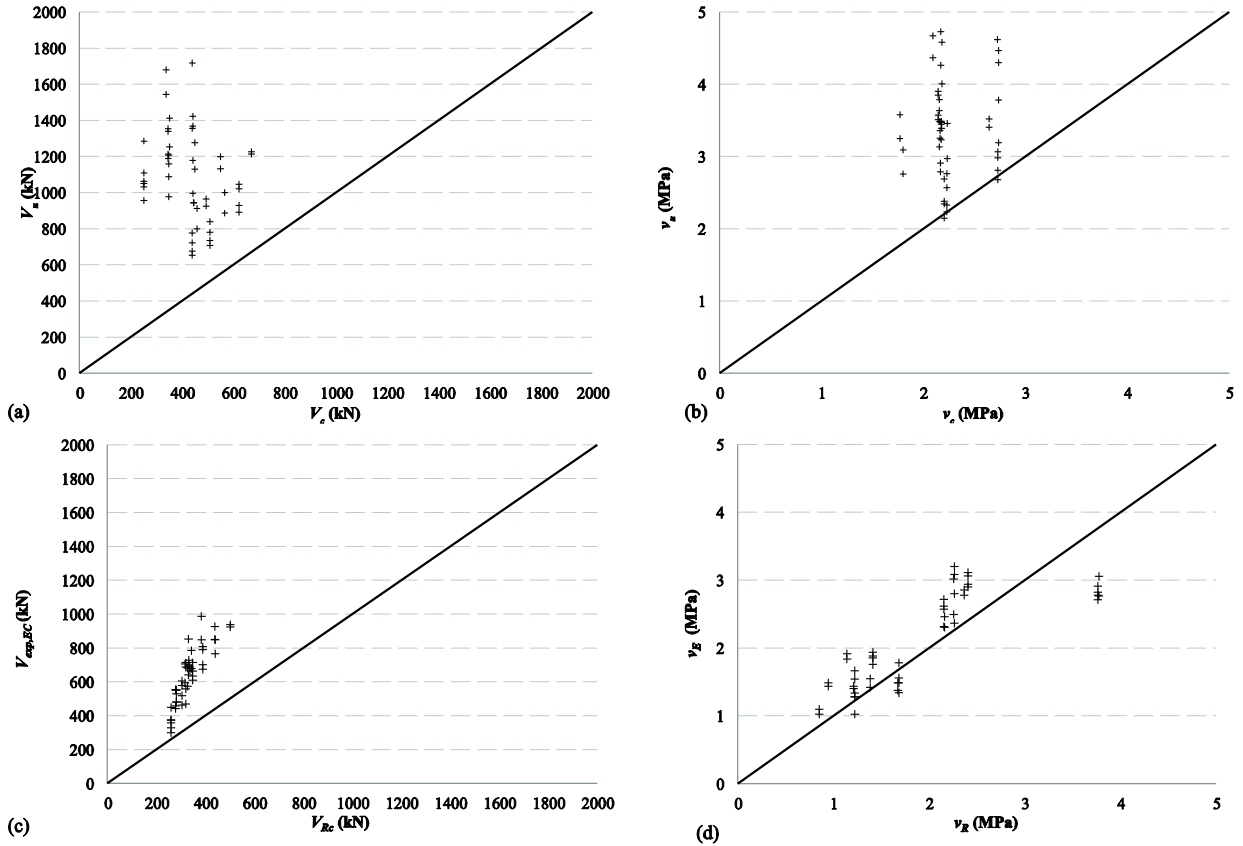
4 5 Figure 3 – Comparison between experiments on asymmetrically loaded slabs and code provisions: (a) 6 ACI 318-14 shear provisions; (b) ACI 318-14 punching provisions; (c) Eurocode 2 shear provisions; (d) 7 Eurocode 2 punching provisions. Conversion: 1 kN = 0.225 kip; 1 MPa = 145 psi. 8
