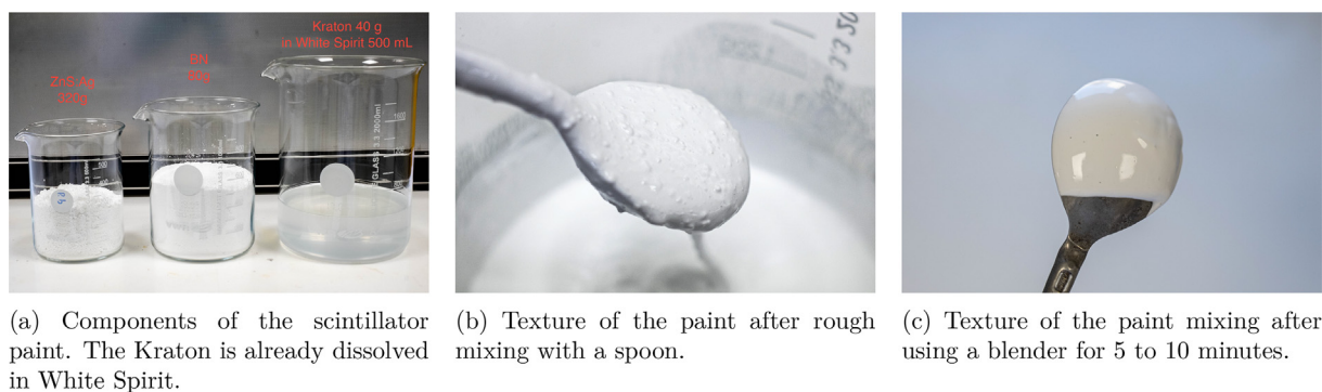
Fig. 2. Scintillator paint mixing.
