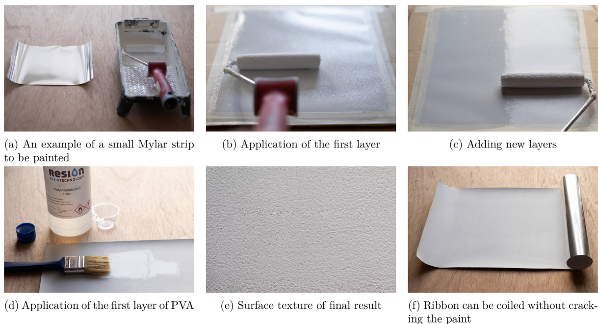
Fig. 3. Ribbon-detector Fabrication.
