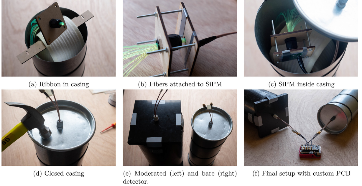
Fig. 6. Casing installment.
