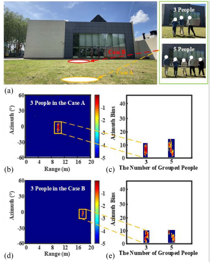
Fig. 3. (a) Video ground truth for three people and five people walking as a group in two cases denoted by A and B. (b) Range–Azimuth map in the case A at about 9 m, with comparison of the detected cells for groups of 3 versus 5 people (c). (d) Range–Azimuth map in the case B at about 16 m, with comparison of the detected cells for groups of 3 versus 5 people (e).
