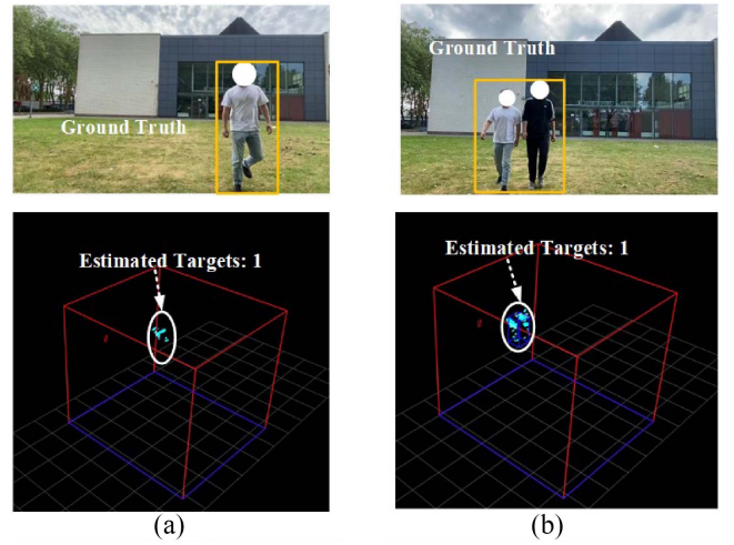
Fig. 12. Visual ground truth and TI 3-D people counting visualizer results when (a) 1 person and (b) 2 people walking as a group are present.
