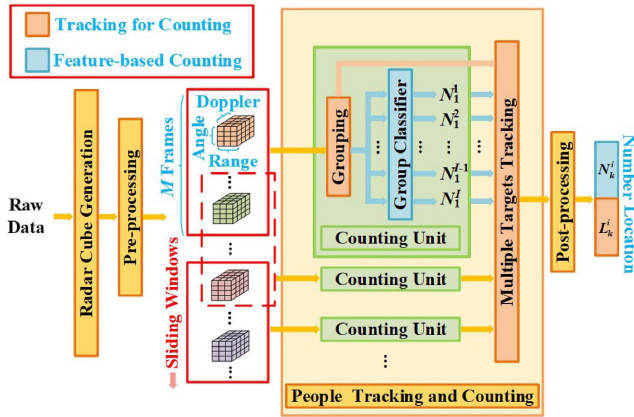
Fig. 6. Overview of the proposed people counting pipeline, which combines relevant elements of the tracking for counting and feature-based counting approaches typically used in isolation in the literature.
