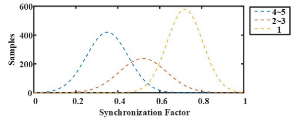
Fig. 5. Distributions of the synchronization factor parameter derived from the CVD for different numbers of grouped people.
