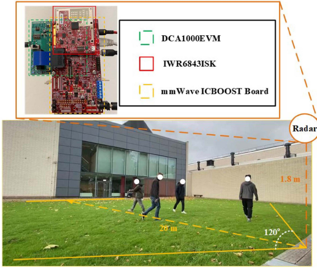
Fig. 9. Radar equipment and scene for the experimental setup to validate the proposed grouped people counting pipeline.
