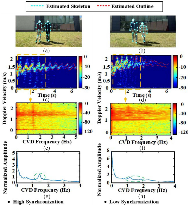
Fig. 4. Analysis of the synchronization for two people walking as a group. Ground truth with estimated skeleton in (a) high synchronization case for people of similar height, and (b) low synchronization case for people of diverse height. Spectrograms for (c) high synchronization and (d) low synchronization case, with Doppler velocity displayed in absolute value. CVD maps in (e) high synchronization and (f) low synchronization case, with CVD profiles in (g) high synchronization and (h) low synchronization case.
