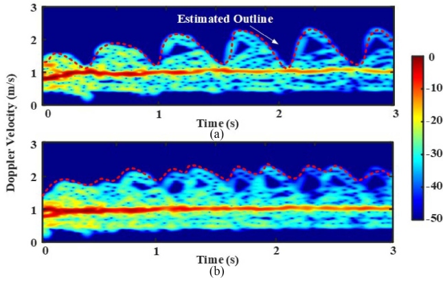
Fig. 2. Simulated spectrograms based on the proposed Group People model when (a) 1 person is walking and (b) 2 people are walking.
