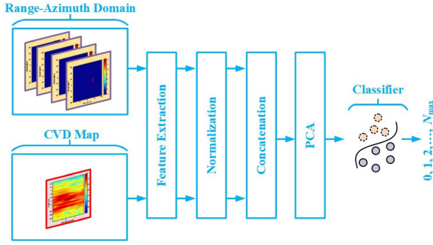
Fig. 7. Overview of the steps for the proposed group classifier.
