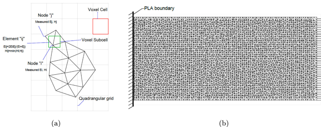
Fig. 3. Lattice model discretization procedure a) and simulated loading condition in uniaxial tensile mode b).
